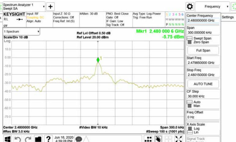
功率密度_BLE_2M_HighCH39-2480
