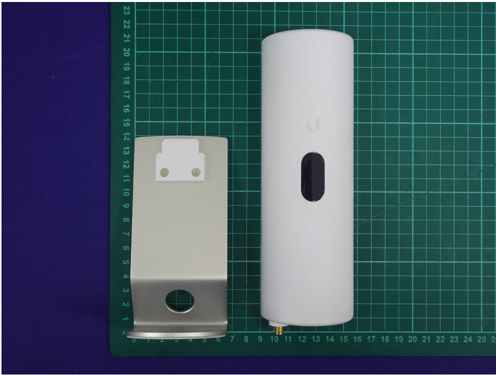
(8) EUT Photo - Trade Name: UBIQUITI, Model No.: U-LTE-Backup Pro
