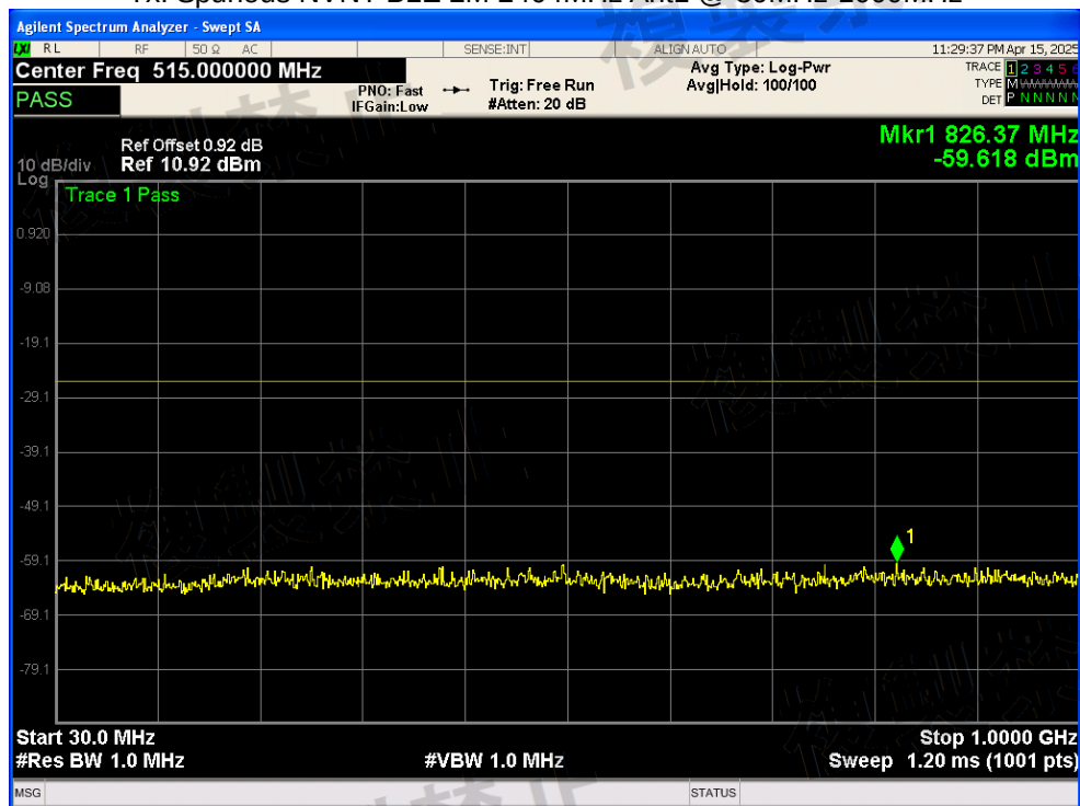
Tx. Spurious NVNT BLE 2M 2404MHz Ant1 @ 30MHz-1000MHz
