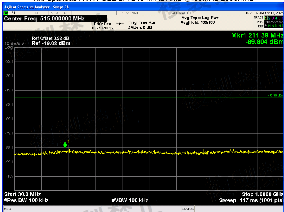
Rx. Spurious NVNT BLE 2M 2404MHz Ant1 @ 30MHz-1000MHz
