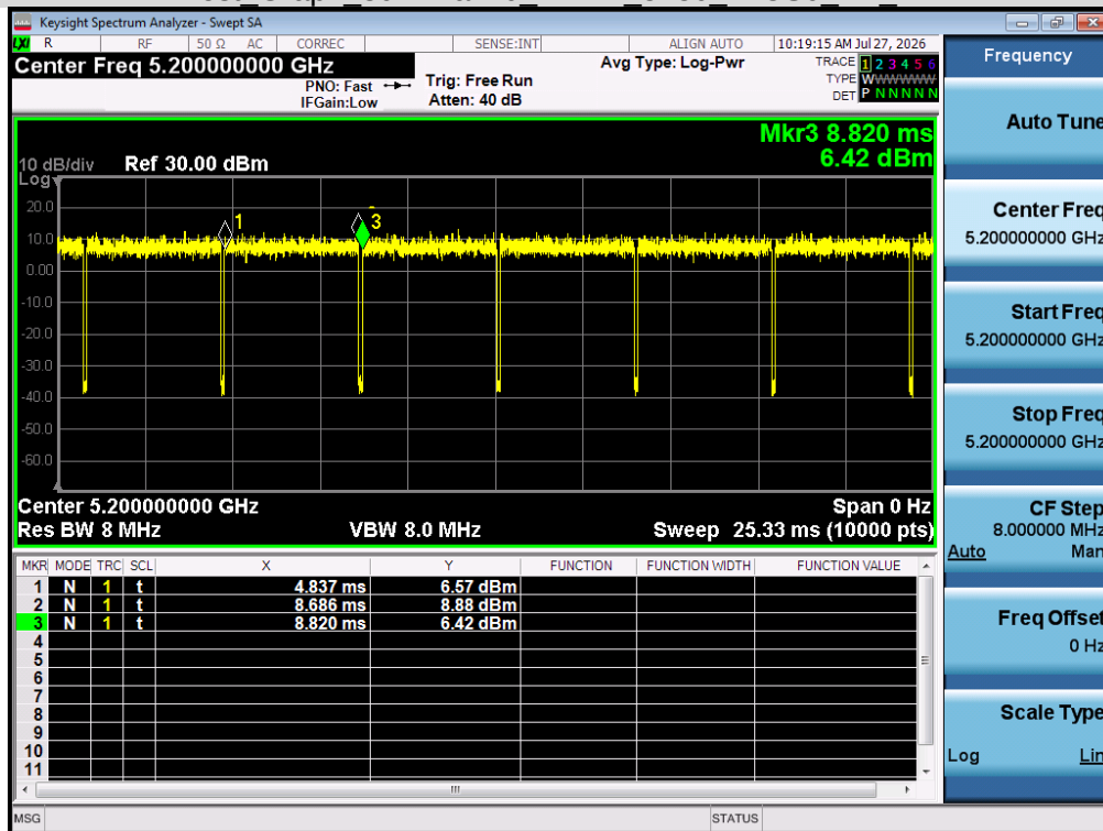
Test Graph 802.11ax20 ANT 1 5200 MCS0 DT NV
