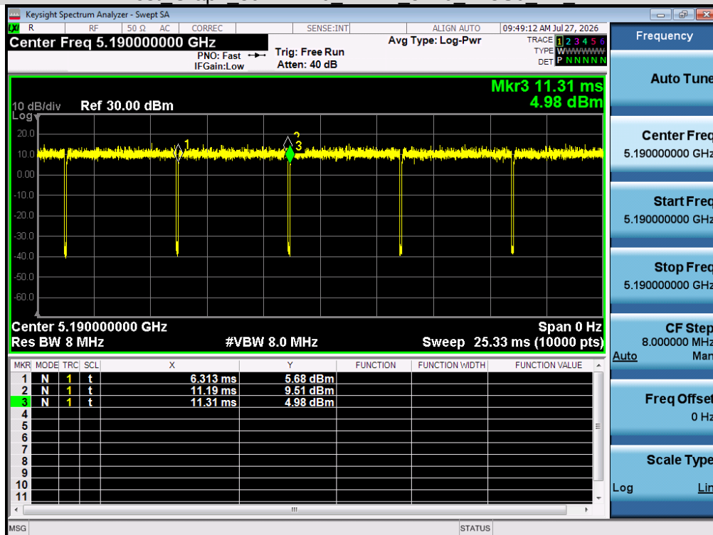
Test Graph 802.11n40 ANT 1 5190 MCS0 DT NV
