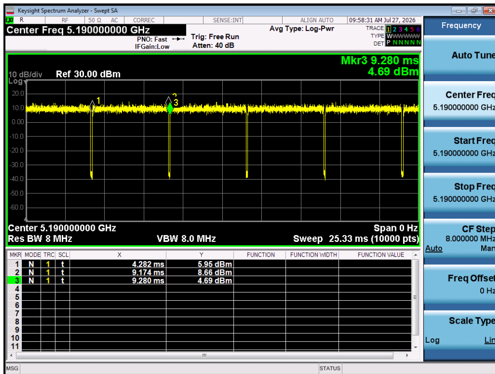
Test Graph 802.11ac40 ANT 1 5190 MCS0 DT NV
