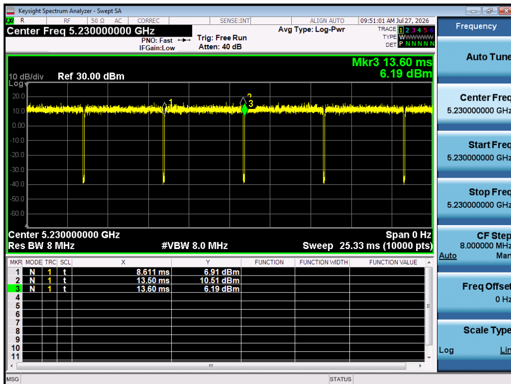
Test Graph 802.11n40 ANT 1 5230 MCS0 DT NV
