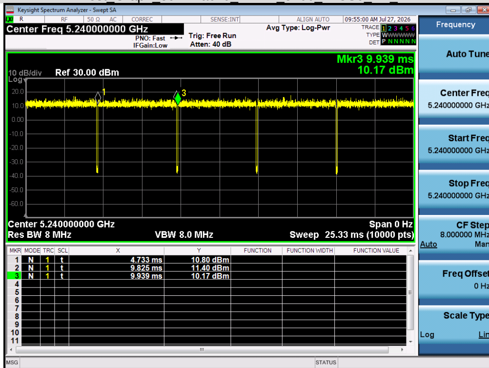
Test_Graph_802.11ac20_ANT 1_5240_MCS0_DT_NV
