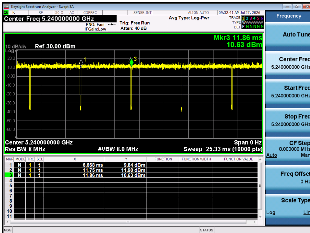
Test Graph 802.11n20 ANT 1 5240 MCS0 DT NV
