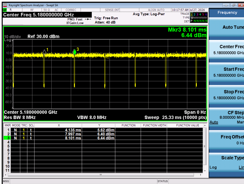
Test Graph 802.11ax20 ANT 1 5180 MCS0 DT NV
