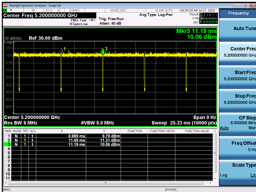
Test Graph 802.11ac20 ANT 1 5200 MCS0 DT NV
