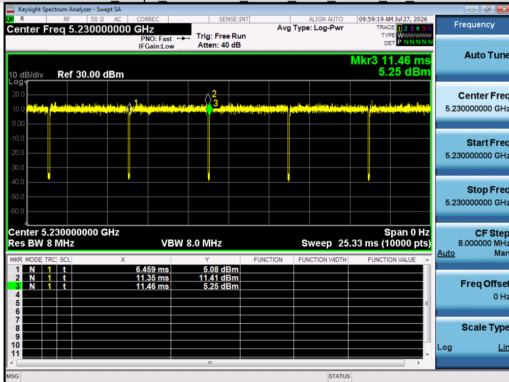
Test_Graph_802.11ac40_ANT 1_5230_MCS0_DT_NV
