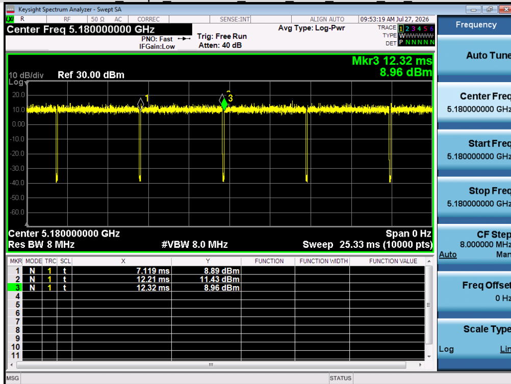
Test Graph 802.11ac20 ANT 1 5180 MCS0 DT NV
