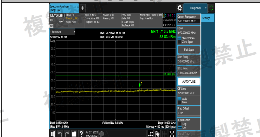
NTNV_BLE_2M_Ant1_2440_30~1000
