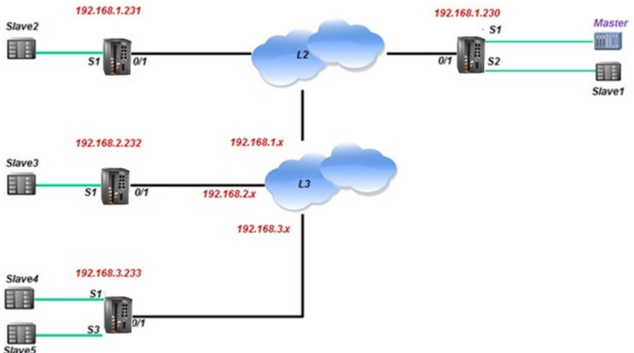
Figure 12 - P2MP Remote Service
