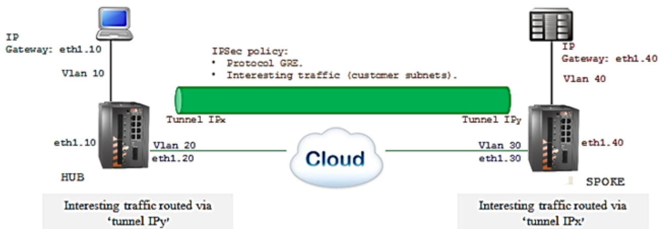
Figure 33 - DM-VPN Topology
