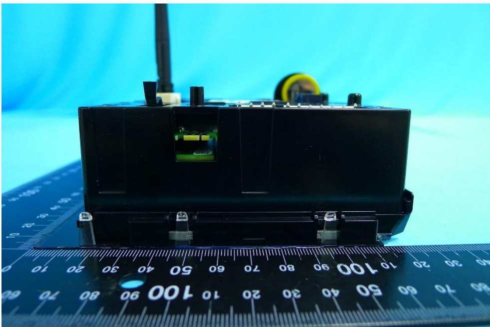
(6) EUT Photo (Touch-5)
