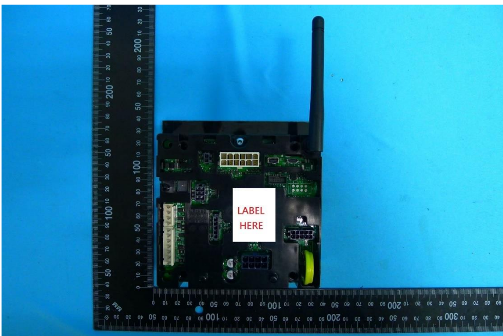
(2) EUT Photo (Touch-5)
