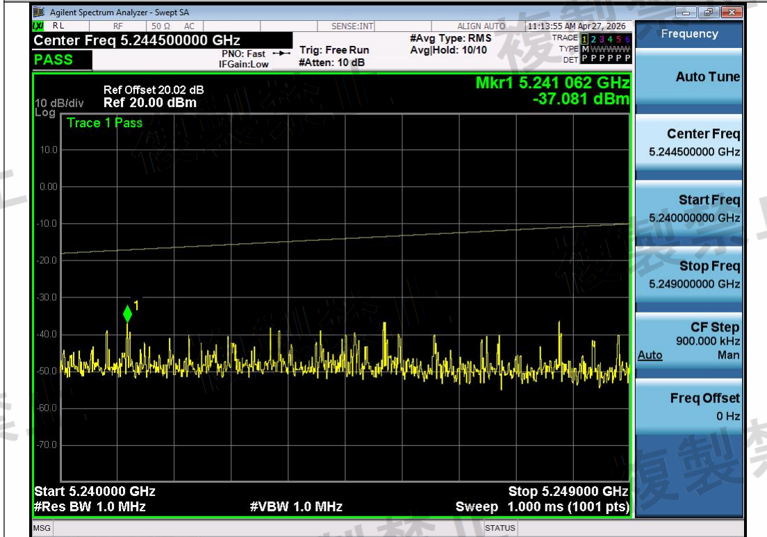
NTNV-11A-Ant1-5280-5240~5249-PASS
