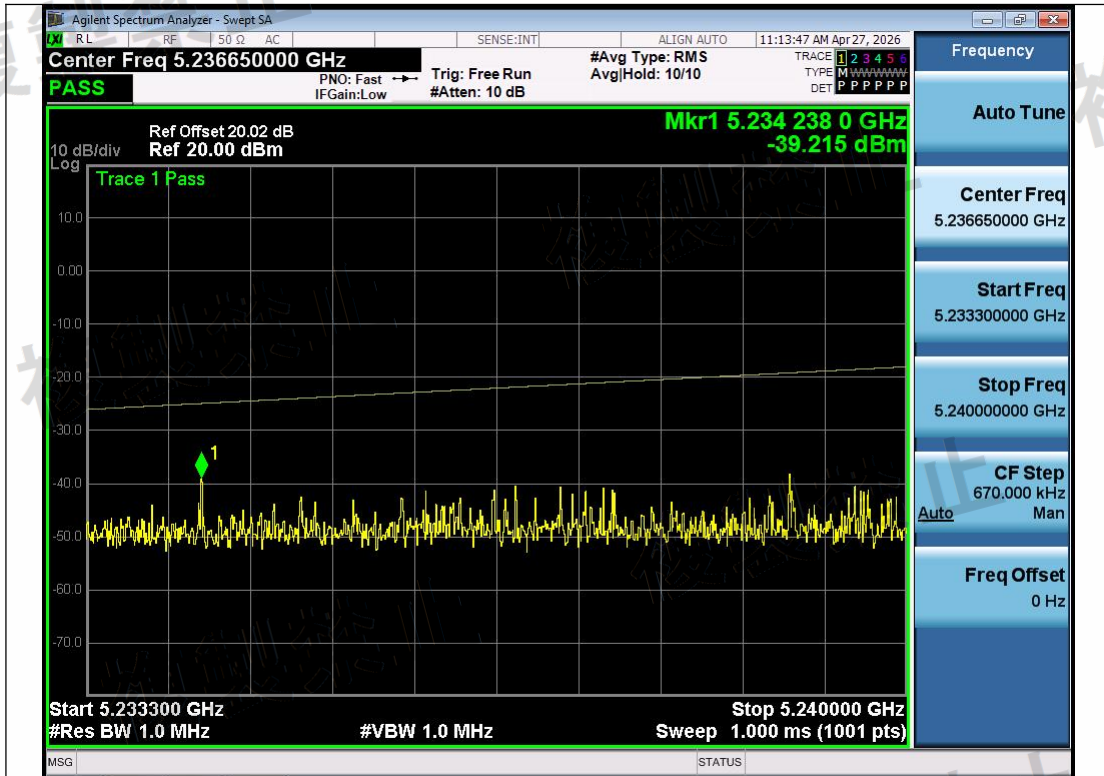
NTNV-11A-Ant1-5280-5233.3~5240-PASS
