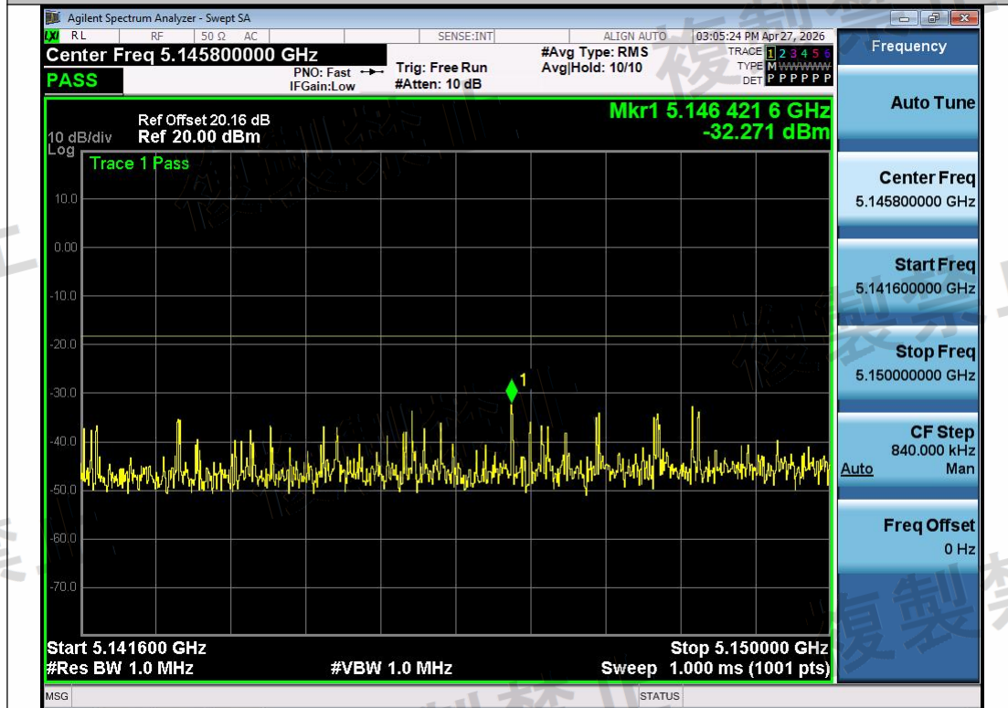
NTNV-11N40SISO-Ant1-5190-5141.6~5150-PASS
