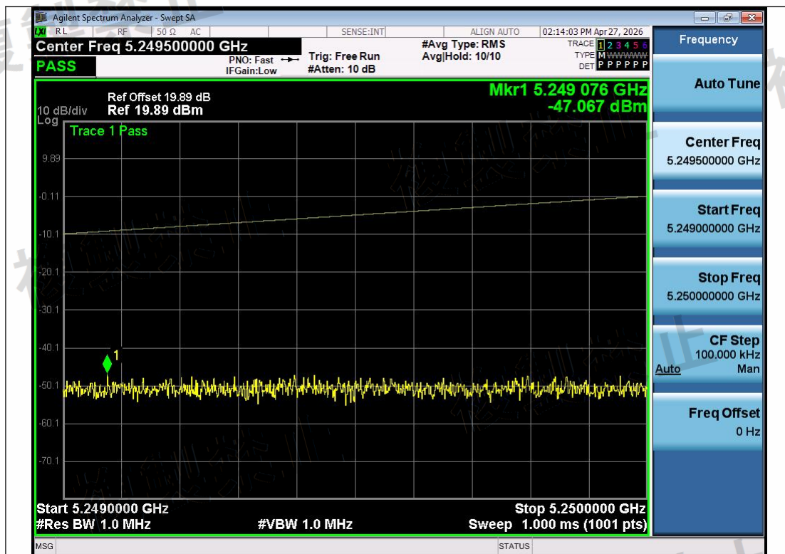
NTNV-11N20SISO-Ant1-5320-5249~5250-PASS
