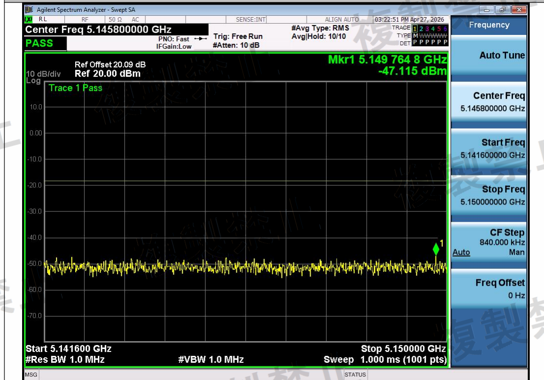
NTNV-11N40SISO-Ant1-5230-5141.6~5150-PASS
