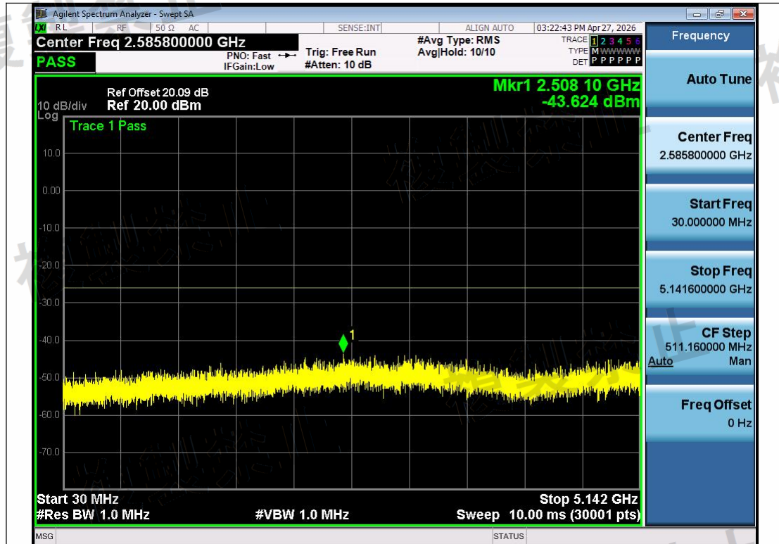
NTNV-11N40SISO-Ant1-5230-30~5141.6-PASS
