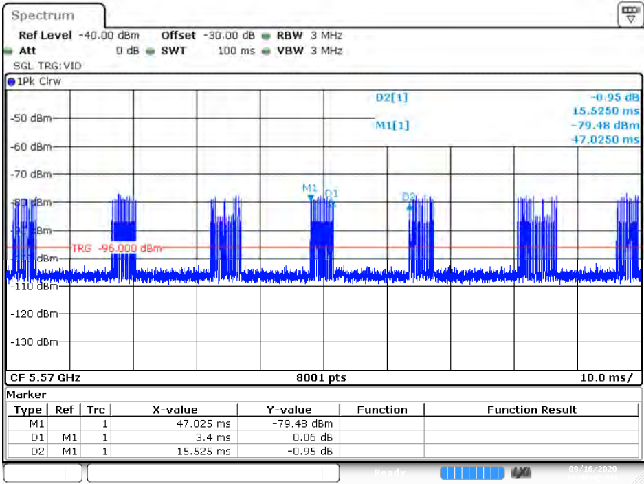
Slave Data Traffic Plot Result Plot of Slave Traffic at 5570MHz
