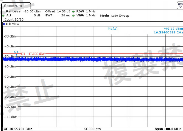
NTNV-11N40-Ant2-5710-1000~26000-PASS
