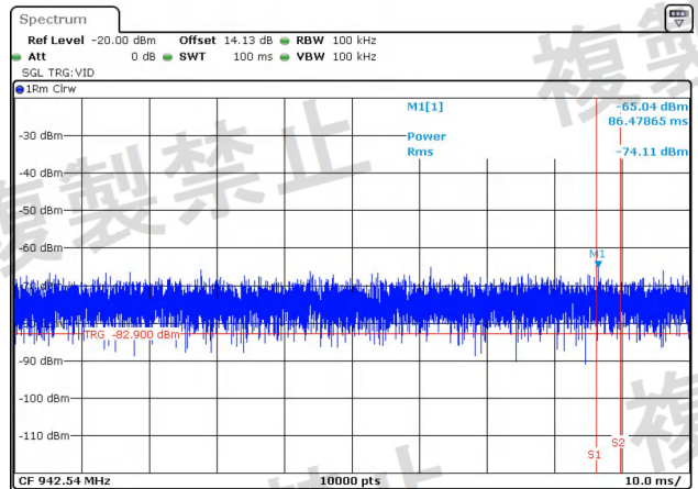
NTNV-11N20MIMO-Ant1-5600-30~1000-PASS
