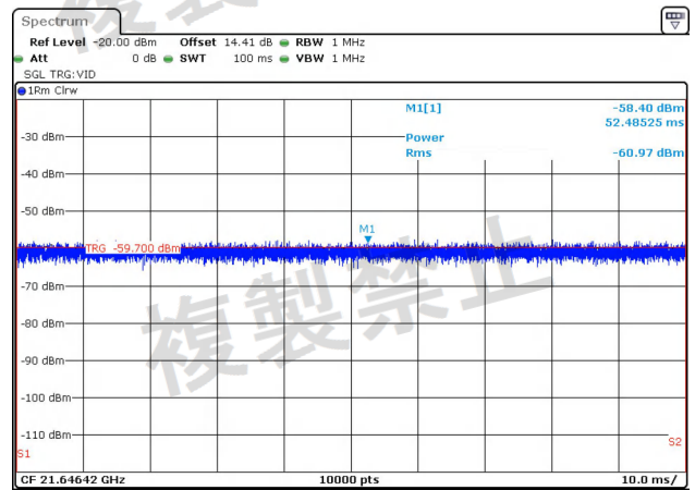
NTNV-11N20-Ant2-5720-1000~26000-PASS
