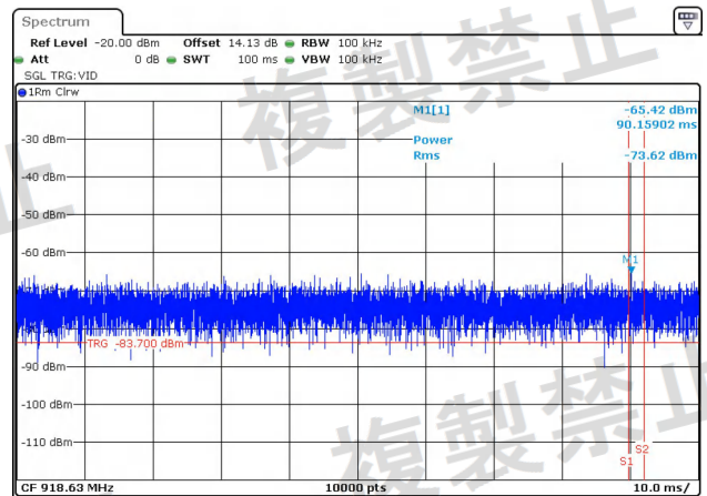
NTNV-11N40-Ant2-5590-30~1000-PASS
