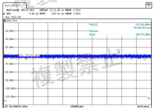
NTNV-11N20MIMO-Ant1-5600-1000~26000-PASS
