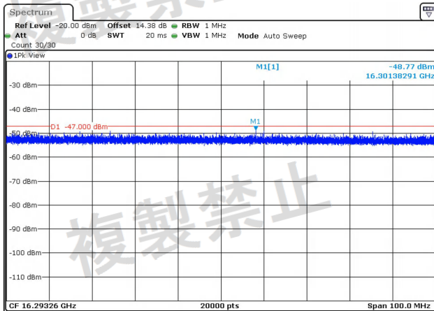
NTNV-11N40MIMO-Ant1-5710-1000~26000-PASS
