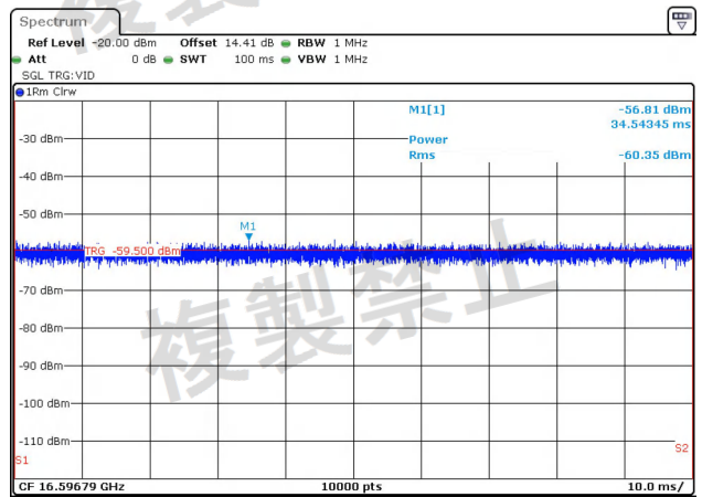
NTNV-11N40-Ant2-5710-1000~26000-PASS
