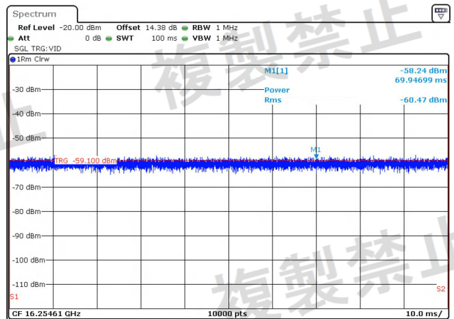
NTNV-11N40-Ant2-5710-1000~26000-PASS
