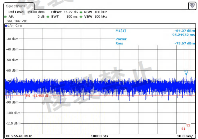
NTNV-11N40MIMO-Ant1-5510-30~1000-PASS
