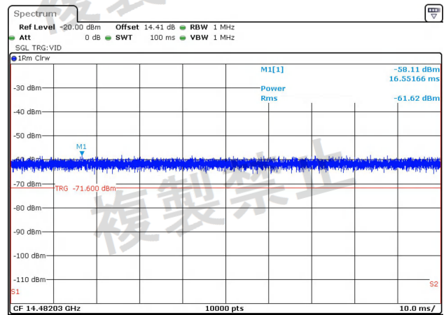
NTNV-11N40MIMO-Ant2-5710-1000~26000-PASS
