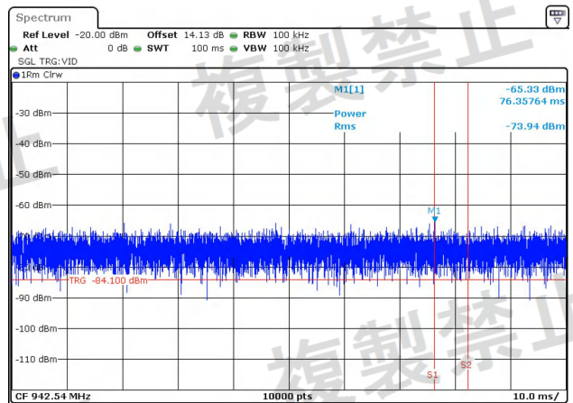
NTNV-11N20MIMO-Ant2-5600-30~1000-PASS
