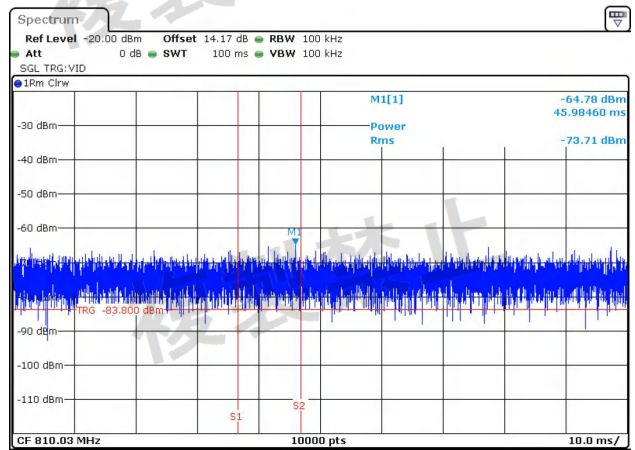
NTNV-11N20MIMO-Ant2-5600-30~1000-PASS
