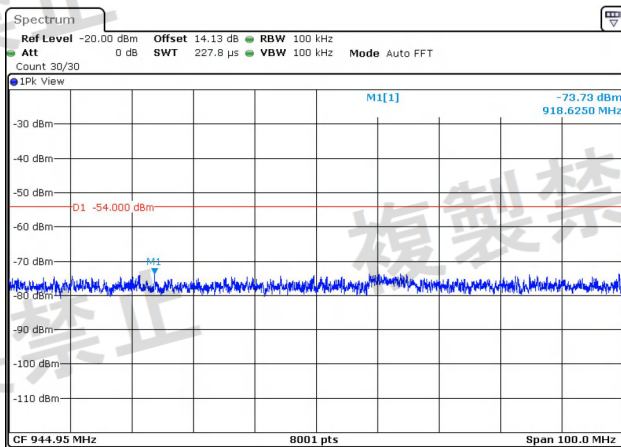
NTNV-11N40-Ant2-5590-30~1000-PASS
