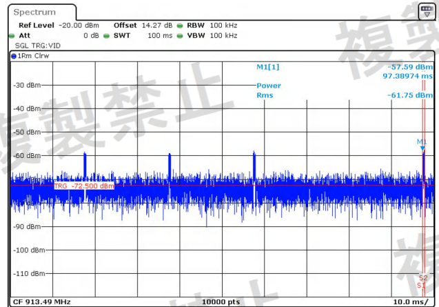
NTNV-11N40-Ant2-5510-30~1000-PASS
