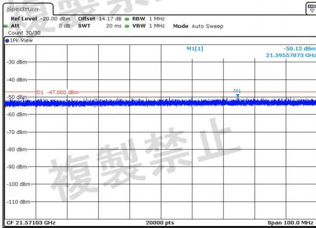
NTNV-11N20-Ant2-5600-1000~26000-PASS
