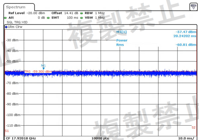
NTNV-11N20MIMO-Ant1-5720-1000~26000-PASS
