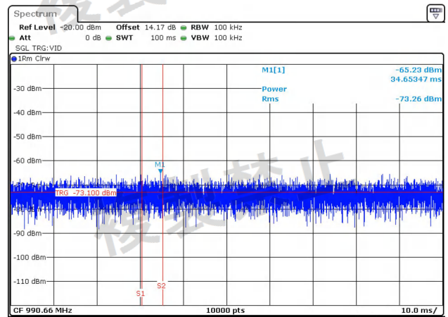
NTNV-11N40-Ant2-5590-30~1000-PASS
