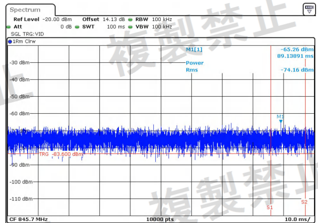
NTNV-11N40MIMO-Ant2-5590-30~1000-PASS
