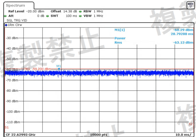
NTNV-11N20MIMO-Ant1-5720-1000~26000-PASS
