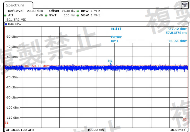
NTNV-11N40MIMO-Ant1-5710-1000~26000-PASS
