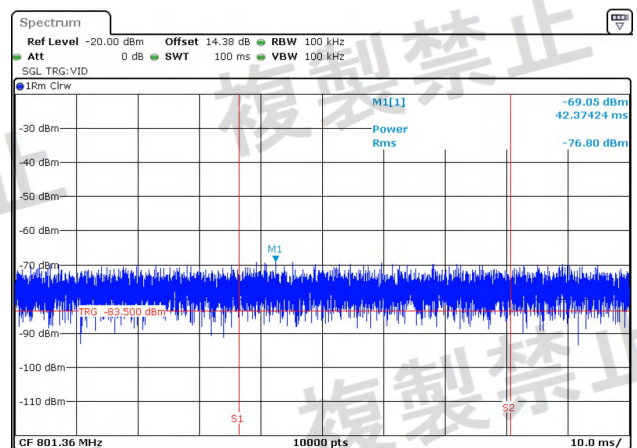
NTNV-11N40MIMO-Ant2-5710-30~1000-PASS
