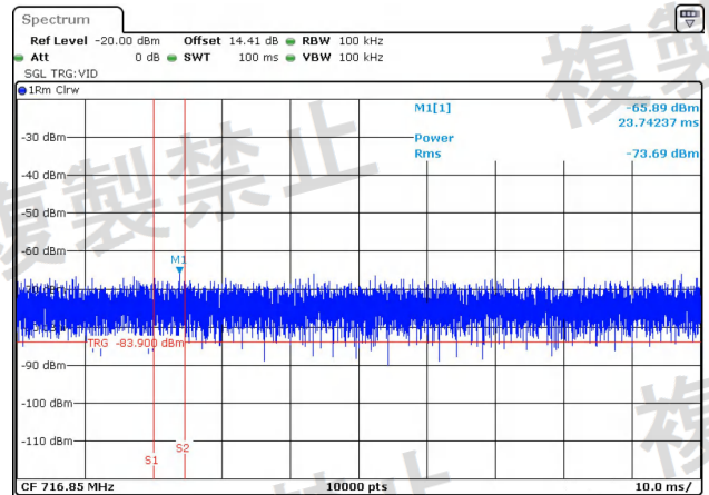
NTNV-11N20MIMO-Ant2-5720-30~1000-PASS
