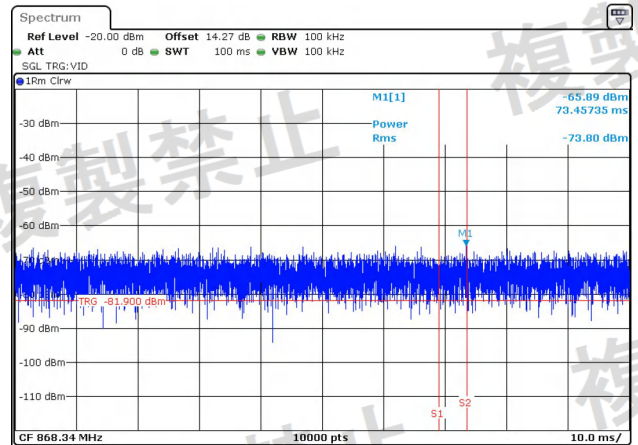
NTNV-11N40MIMO-Ant2-5510-30~1000-PASS
