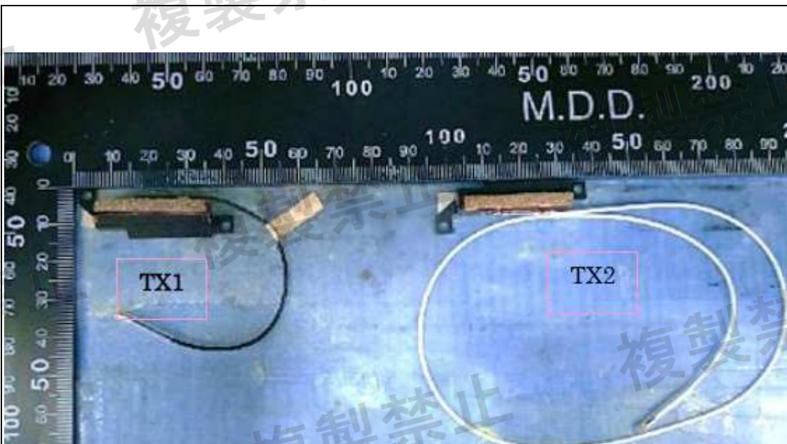
Antenna 2. AYF6Y-100048 (1415-088P000) (Main) & AYF6Y-100049 (1415-088H000) (Aux), AWAN, 2021/6/15
