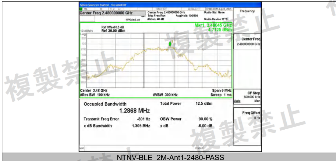
NTNV-BLE_2M-Ant1-2480-PASS
