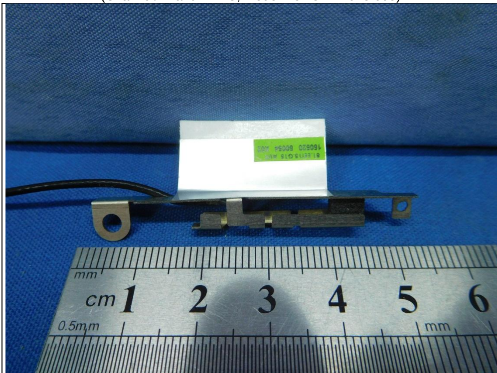
Antenna Set 1 (Chain 0 / Brand: WNC; Model No.: 81-EBJ15.005)
