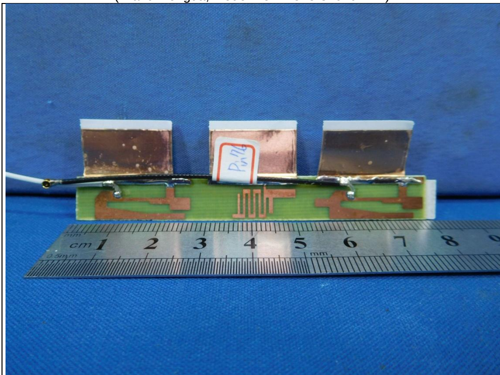
Antenna Set 2 (Brand: Tongda; Model No.: T-543-8201044-A)
