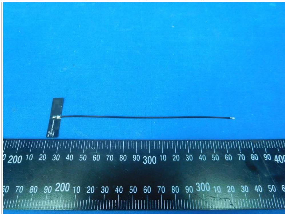
Antenna Set 6 Brand: Molex / Model No.: 1461531150
