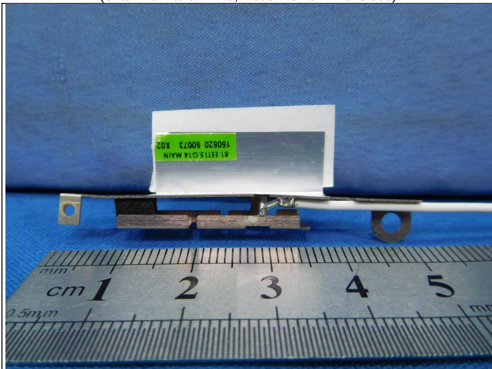
Antenna Set 1 (Chain 1 / Brand: WNC; Model No.: 81-EBJ15.005)
