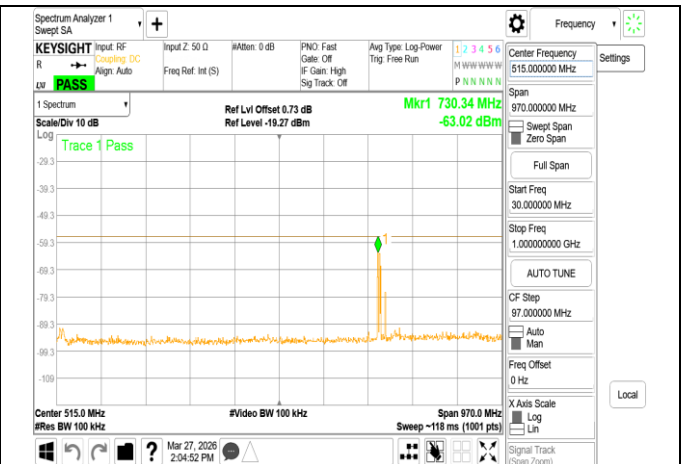
VLP 802.11n 40MHz Chain0 6405MHz Range1
