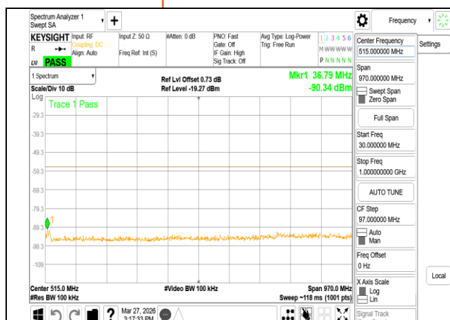
VLP 802.11ax 80MHz Chain0 5985MHz Range1
