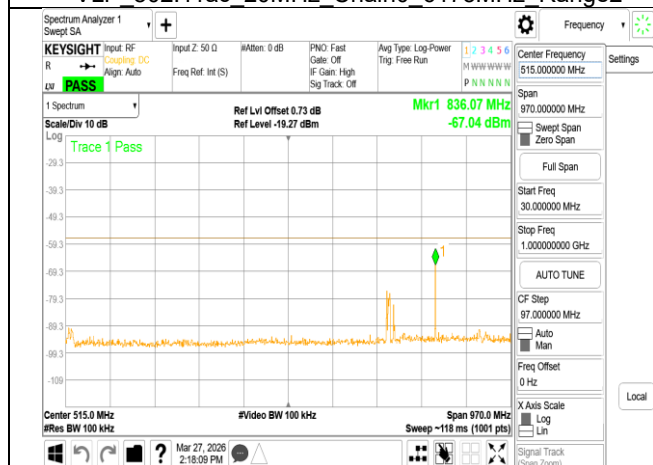
VLP_802.11ac_20MHz_Chain0_6415MHz_Range1
