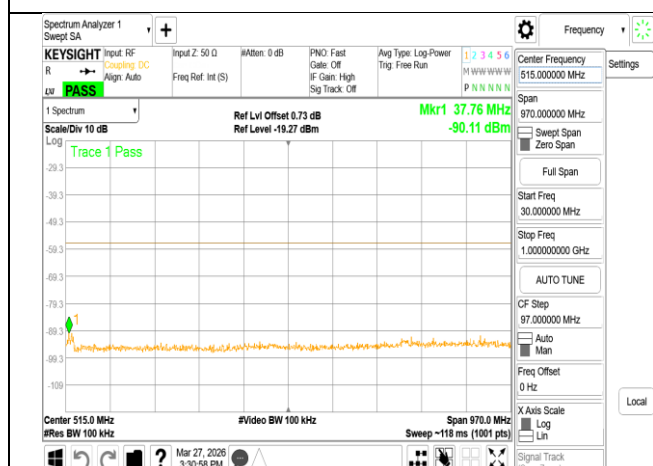
VLP_802.11ax_160MHz_Chain0_6345MHz_Range1
