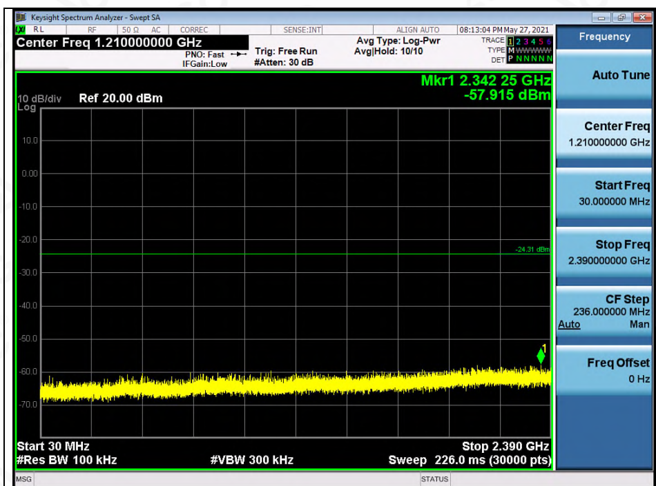
Test_Graph_EDR_ANT1_2402_2Mbps_Lower Band Emissions
