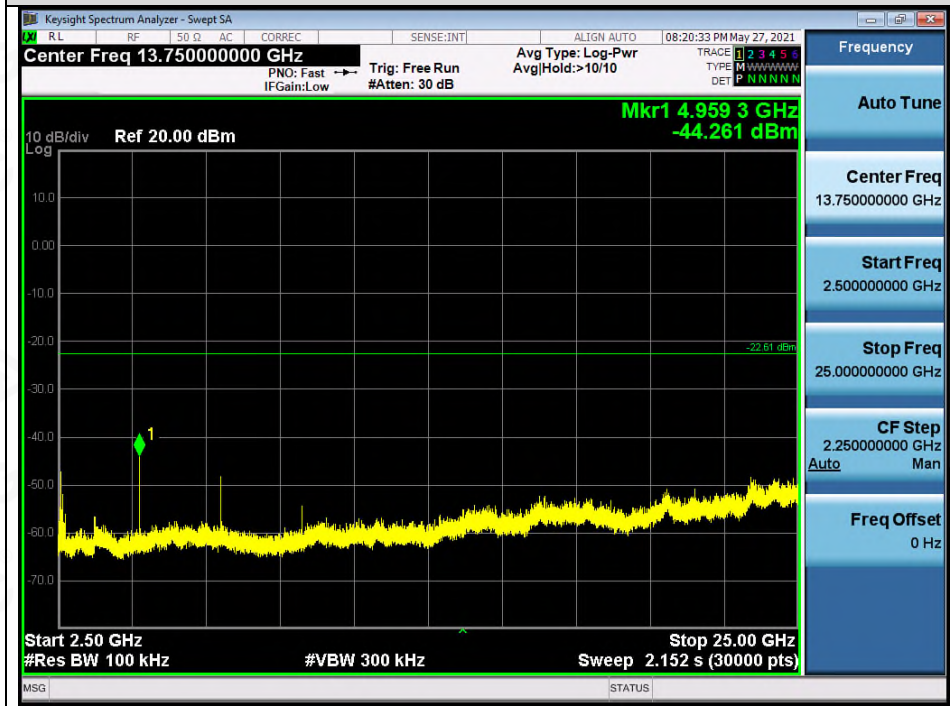
Test_Graph_EDR_ANT1_2480_2Mbps_Higher Band Emissions
