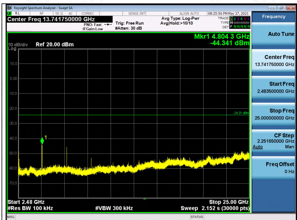
Test_Graph_EDR_ANT1_2402_3Mbps_Higher Band Emissions
