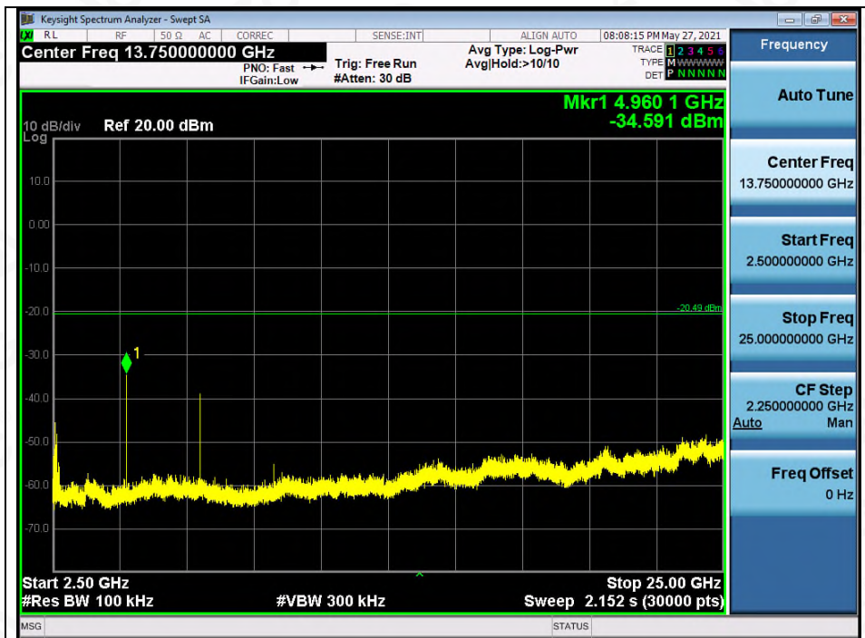
Test_Graph_BR_ANT1_2480_1Mbps_Higher Band Emissions
