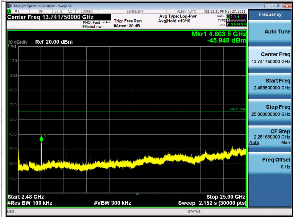
Test_Graph_EDR_ANT1_2402_2Mbps_Higher Band Emissions
