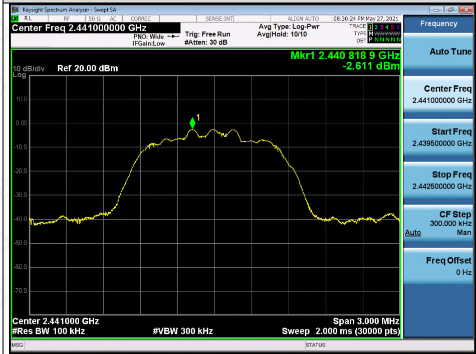
Test_Graph_EDR_ANT1_2441_3Mbps_Reference Level
