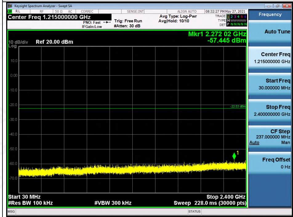
Test_Graph_EDR_ANT1_2480_3Mbps_Lower Band Emissions
