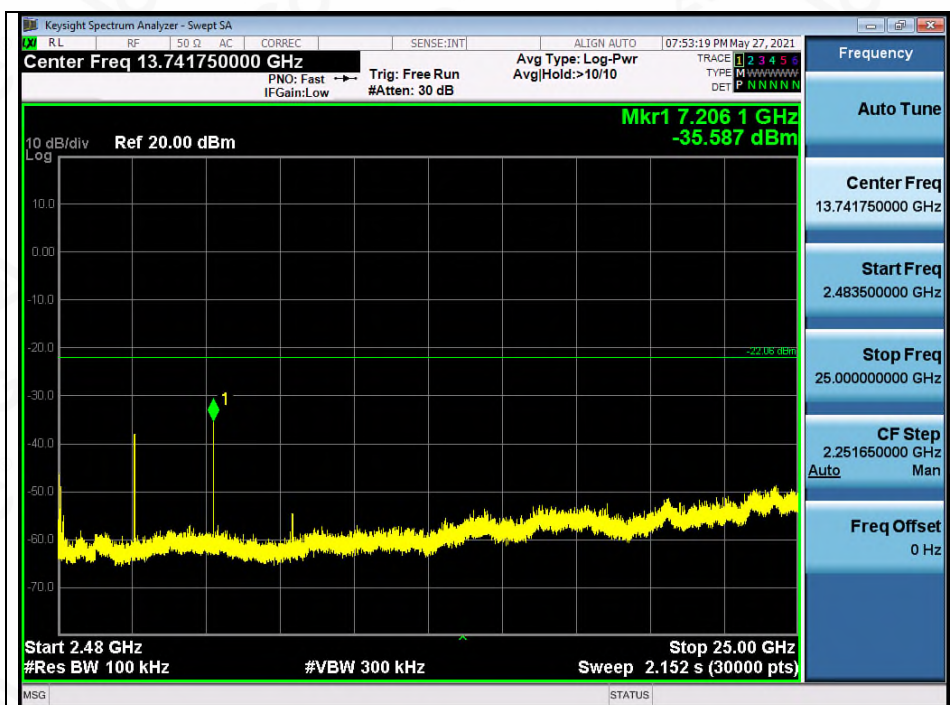
Test_Graph_BR_ANT1_2402_1Mbps_Higher Band Emissions
