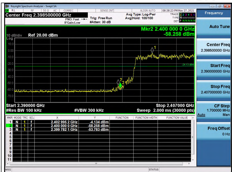
Test_Graph_EDR_HOP_ANT1_NA_3Mbps_Lower Band Edge Emissions
