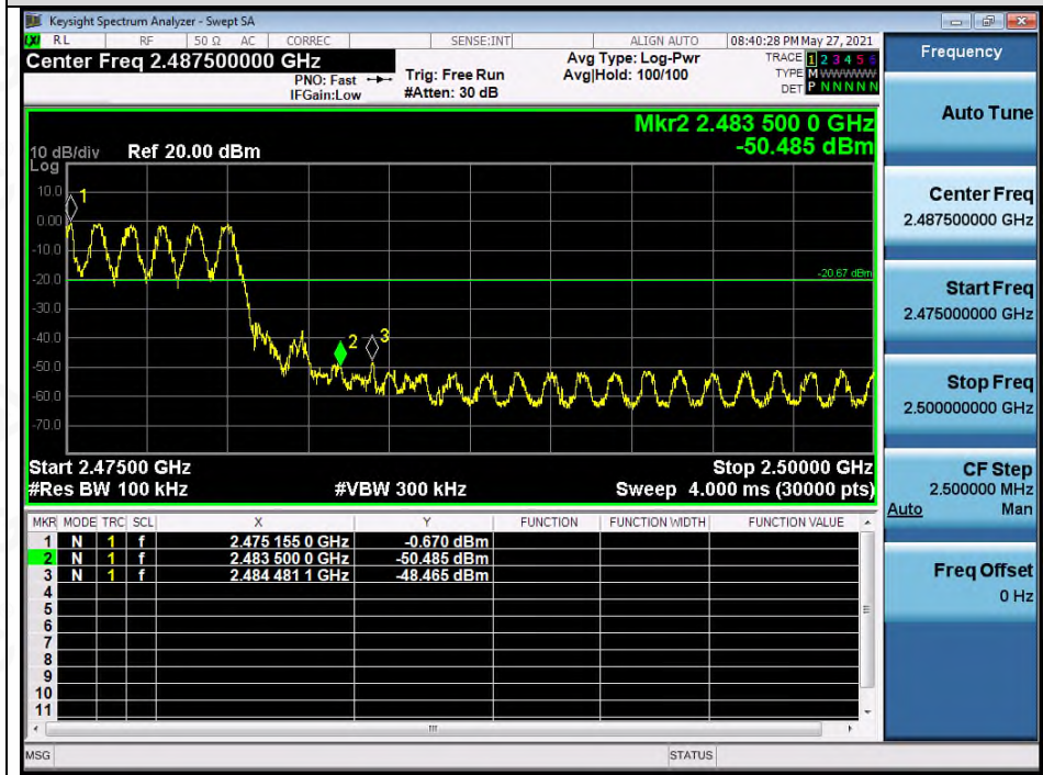
Test_Graph_BR_HOP_ANT1_NA_1Mbps_Higher Band Edge Emissions
