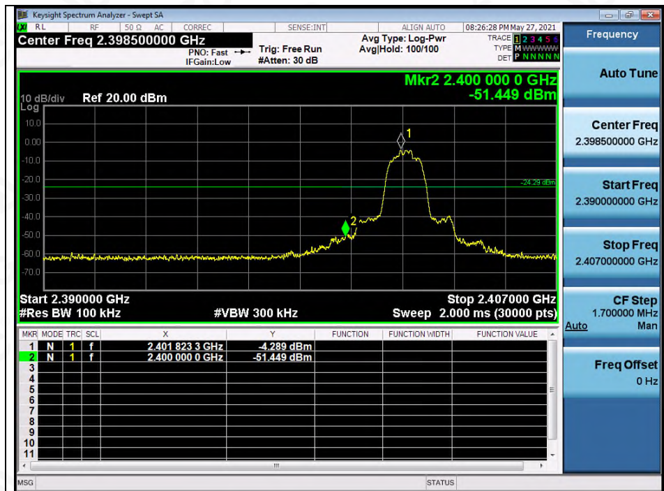
Test_Graph_EDR_ANT1_2402_3Mbps_Lower Band Edge Emissions
