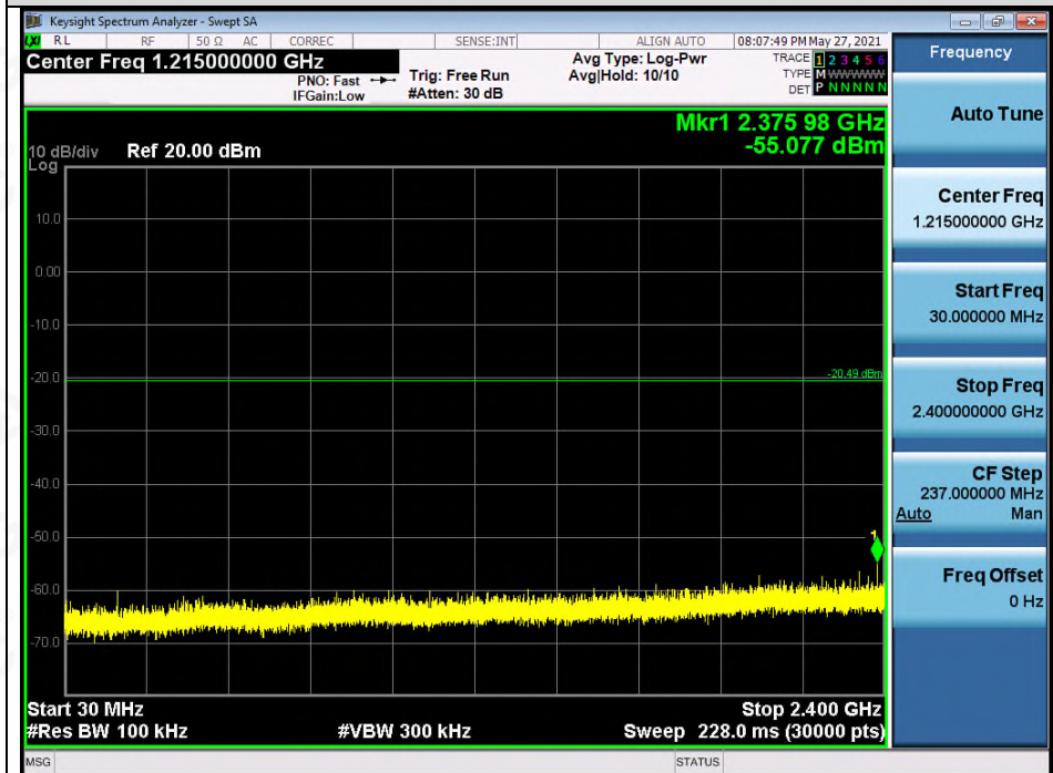
Test_Graph_BR_ANT1_2480_1Mbps_Lower Band Emissions
