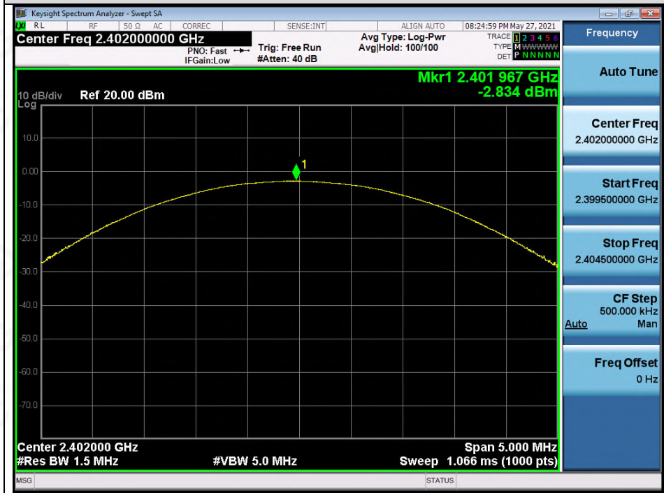
Test_Graph_EDR_ANT1_2402_3Mbps_Peak Power
