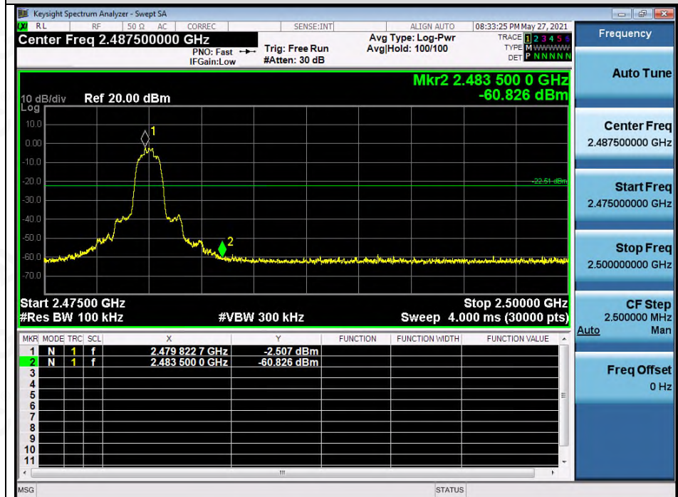
Test_Graph_EDR_ANT1_2480_3Mbps_Higher Band Edge Emissions
