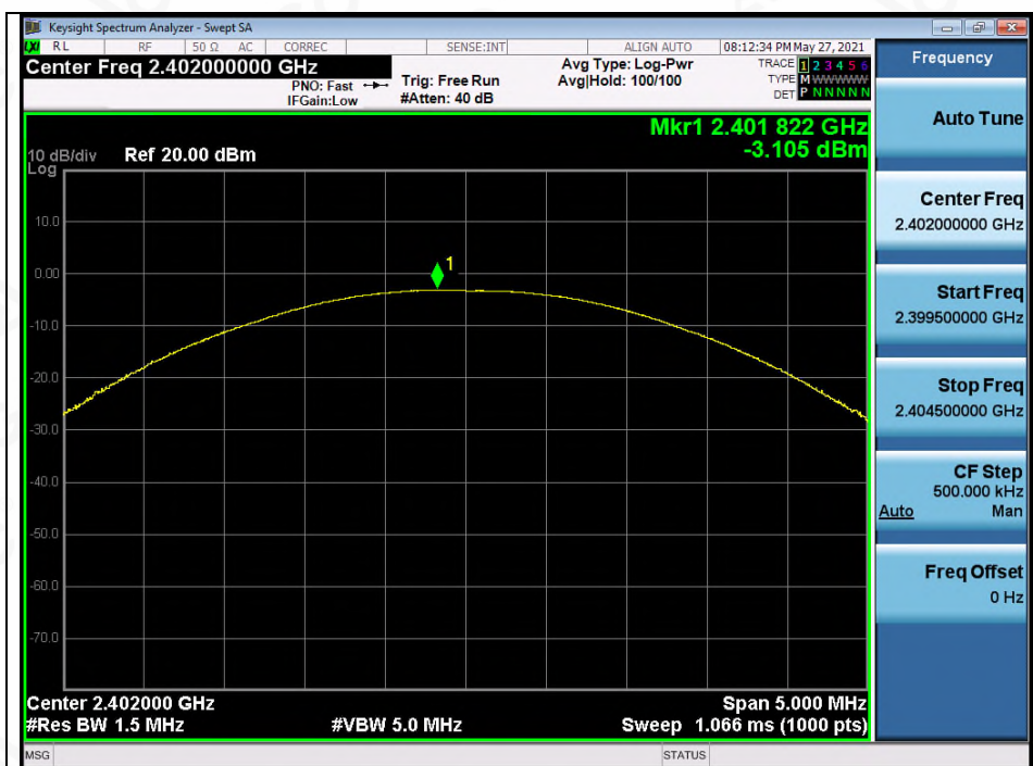
Test_Graph_EDR_ANT1_2402_2Mbps_Peak Power
