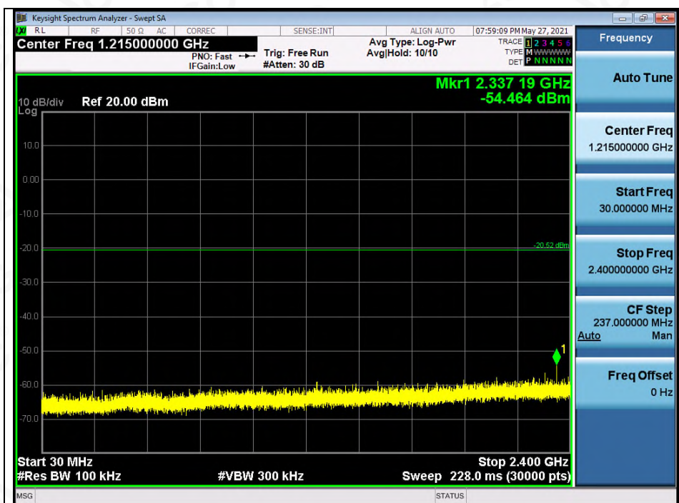
Test_Graph_BR_ANT1_2441_1Mbps_Lower Band Emissions
