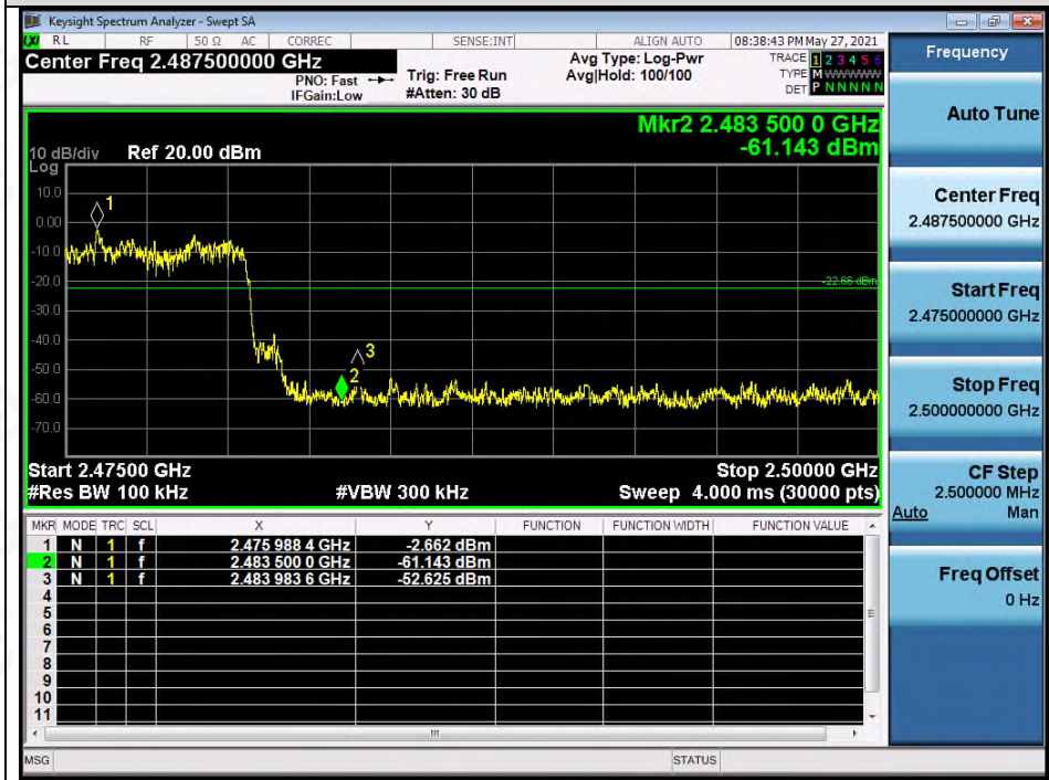
Test_Graph_EDR_HOP_ANT1_NA_3Mbps_Higher Band Edge Emissions
