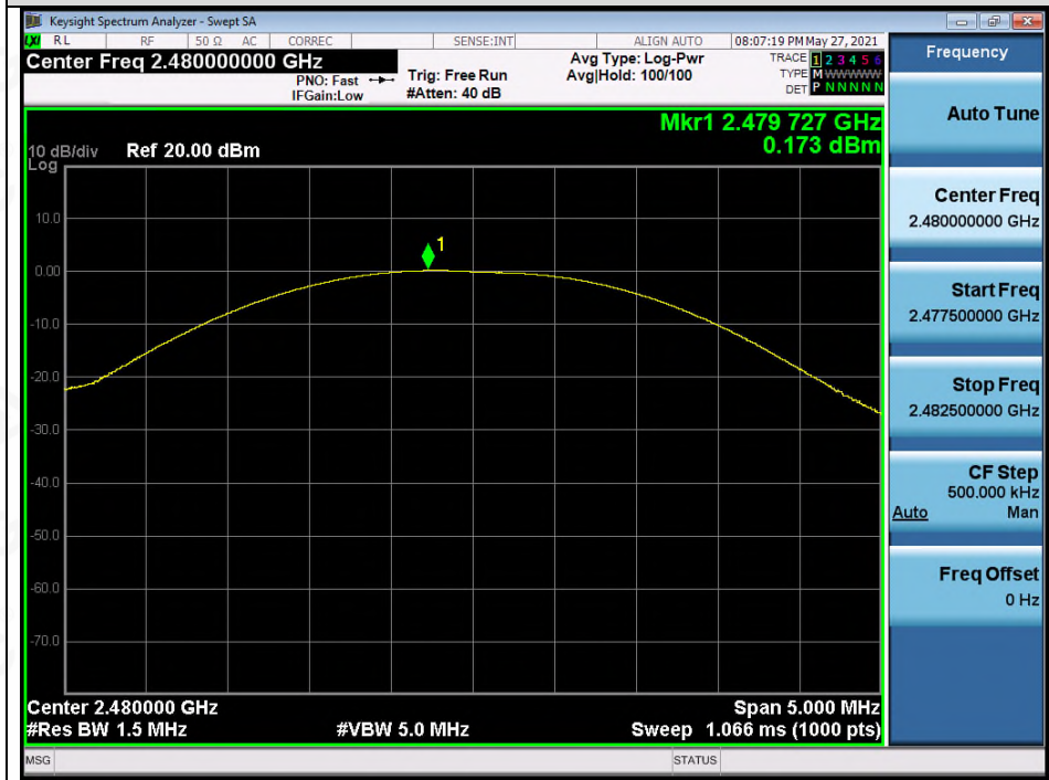
Test_Graph_BR_ANT1_2480_1Mbps_Peak Power
