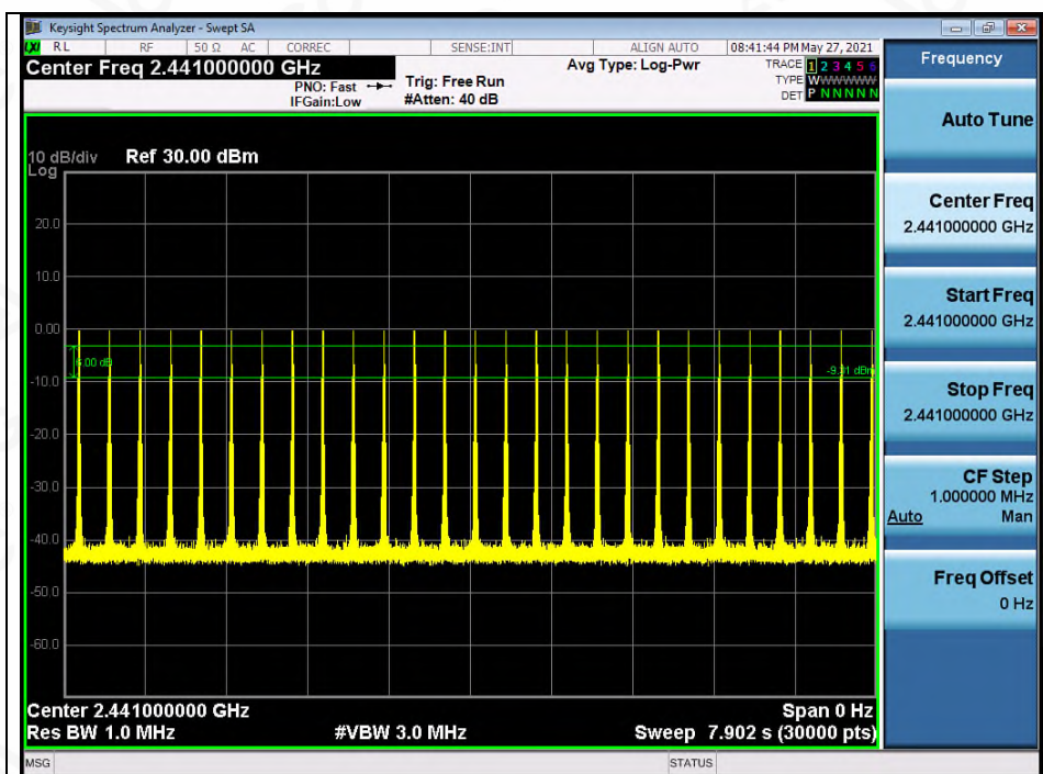
Test_Graph_BR_HOP_ANT1_NA_1Mbps_2441_Number of Burst
