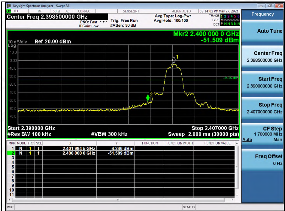
Test_Graph_EDR_ANT1_2402_2Mbps_Lower Band Edge Emissions
