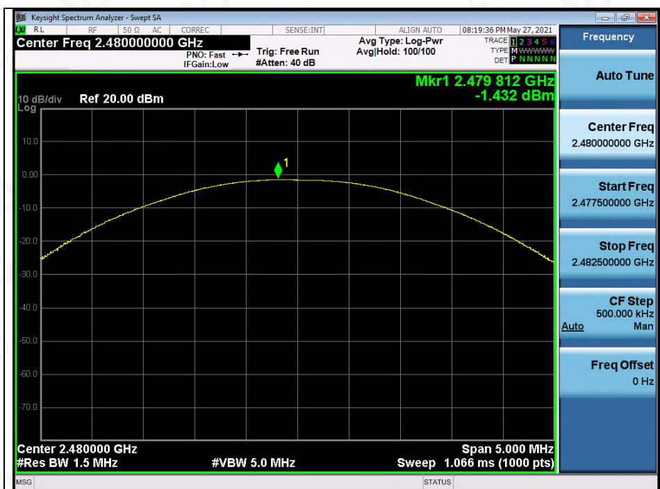
Test_Graph_EDR_ANT1_2480_2Mbps_Peak Power
