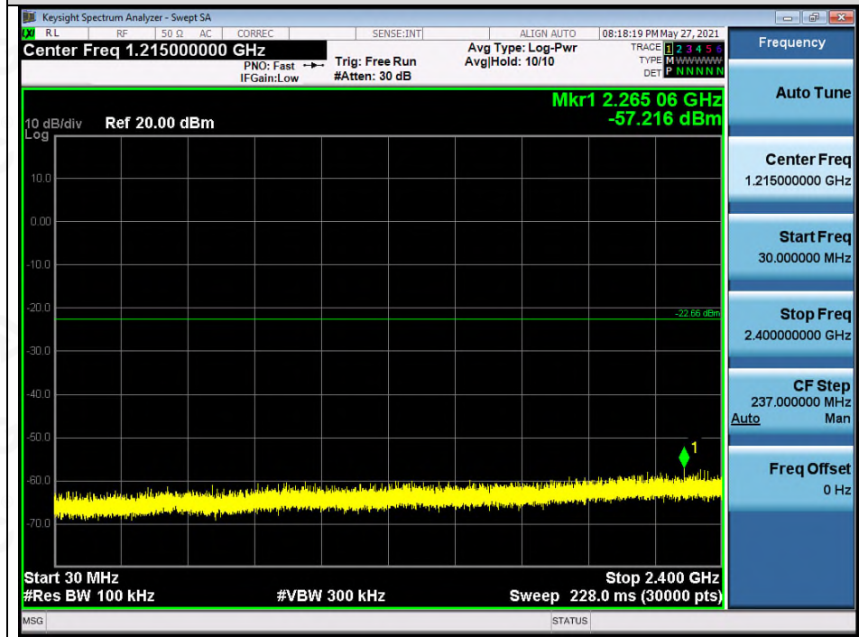
Test_Graph_EDR_ANT1_2441_2Mbps_Lower Band Emissions
