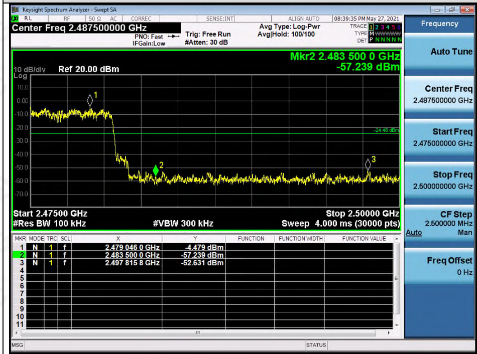
Test_Graph_EDR_HOP_ANT1_NA_2Mbps_Higher Band Edge Emissions
