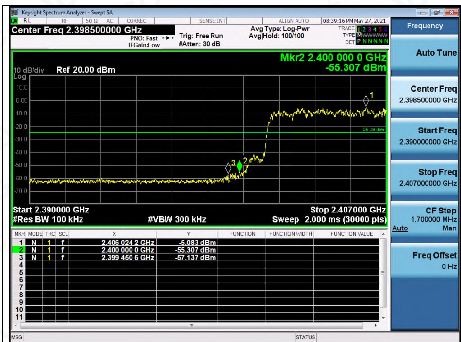
Test_Graph_EDR_HOP_ANT1_NA_2Mbps_Lower Band Edge Emissions
