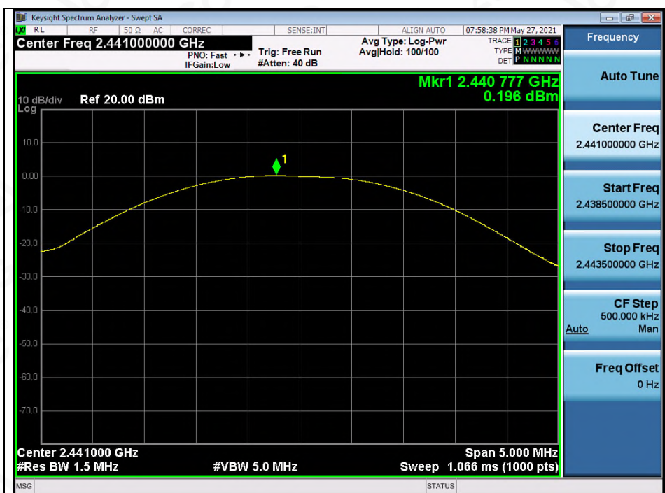
Test_Graph_BR_ANT1_2441_1Mbps_Peak Power
