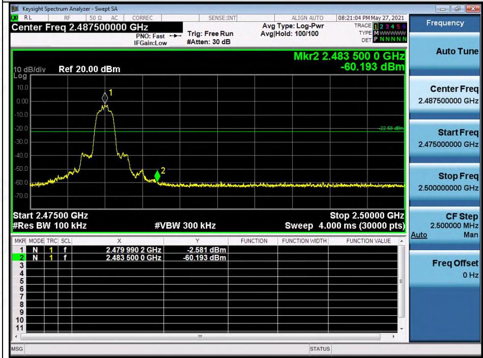
Test_Graph_EDR_ANT1_2480_2Mbps_Higher Band Edge Emissions
