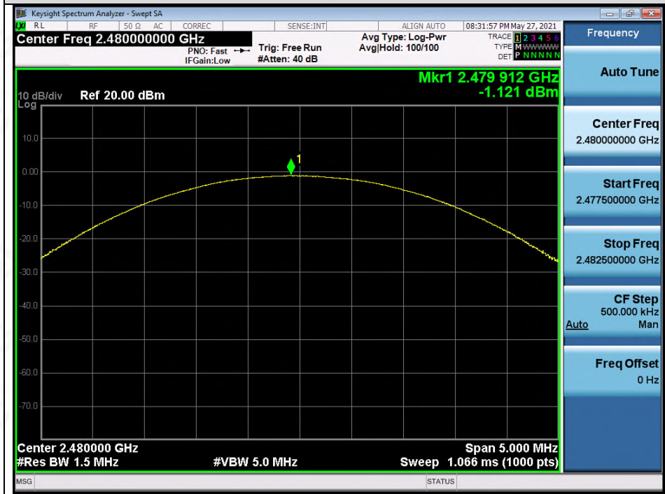
Test_Graph_EDR_ANT1_2480_3Mbps_Peak Power
