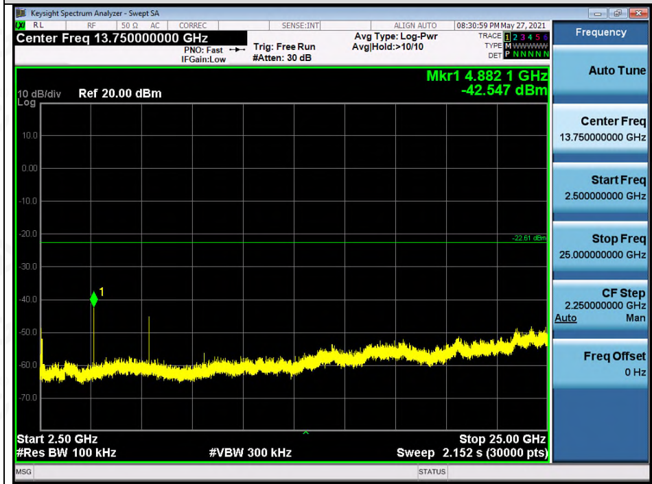
Test_Graph_EDR_ANT1_2441_3Mbps_Higher Band Emissions
