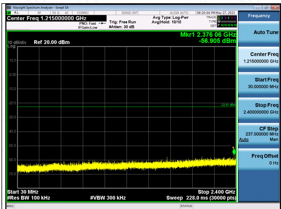
Test_Graph_EDR_ANT1_2480_2Mbps_Lower Band Emissions
