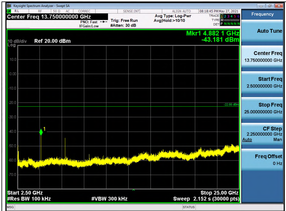
Test_Graph_EDR_ANT1_2441_2Mbps_Higher Band Emissions
