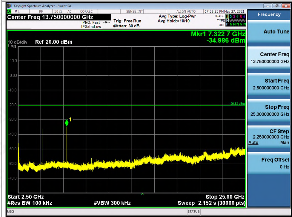
Test_Graph_BR_ANT1_2441_1Mbps_Higher Band Emissions
