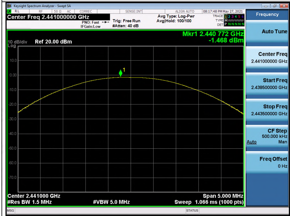
Test_Graph_EDR_ANT1_2441_2Mbps_Peak Power
