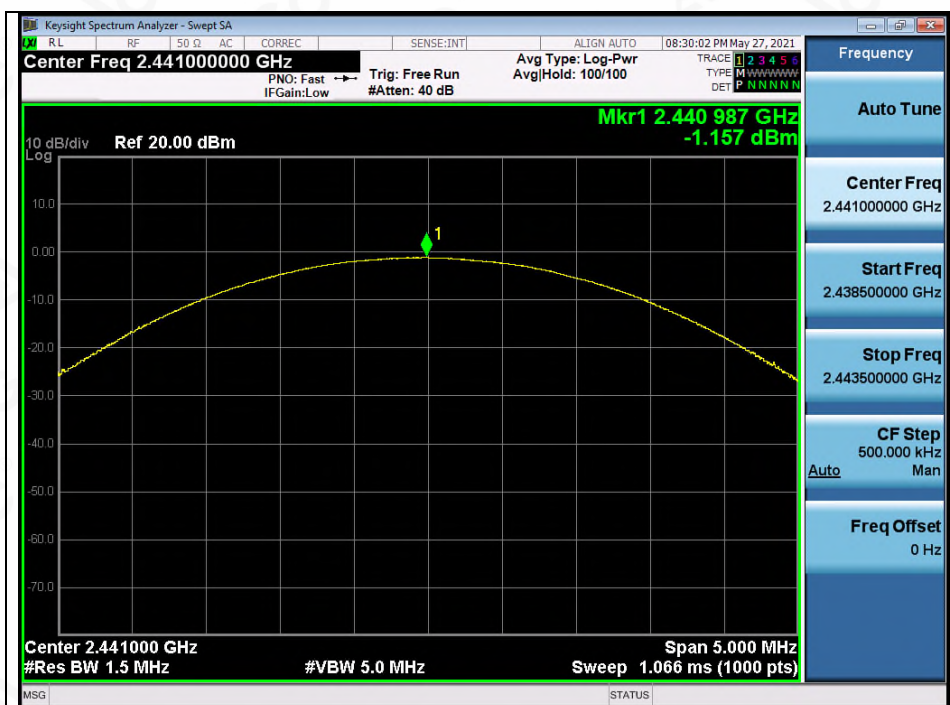
Test_Graph_EDR_ANT1_2441_3Mbps_Peak Power
