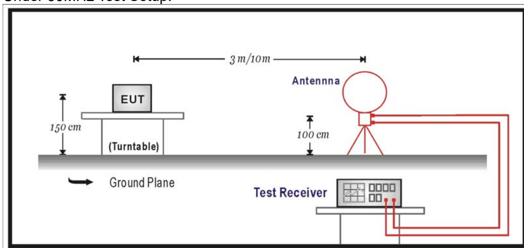
Under 1GHz Test Setup:
