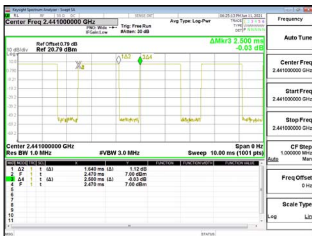
GFSK_1M_DH5_2441MHz
