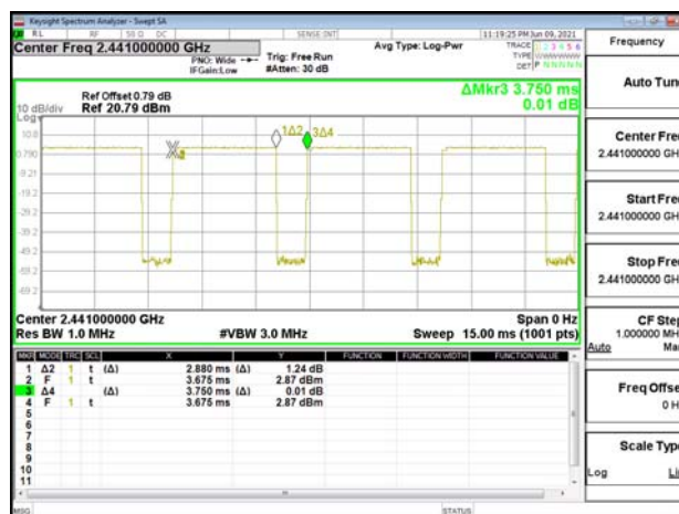
4DQPSK_2M_DH5_2441MHz
