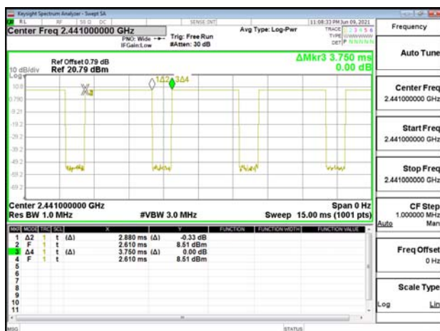
GFSK_1M_DH5_2441MHz
