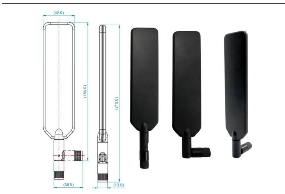
Antenna No. 27
