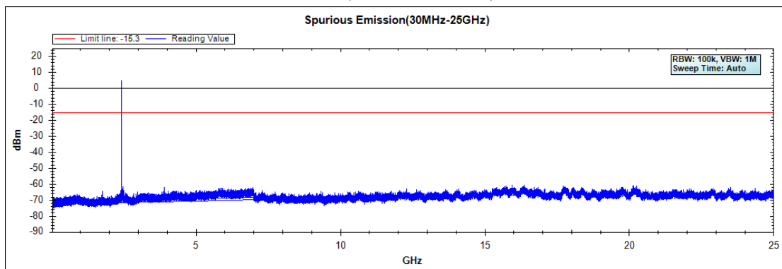
Channel 39 (30MHz-25GHz)-GFSK
