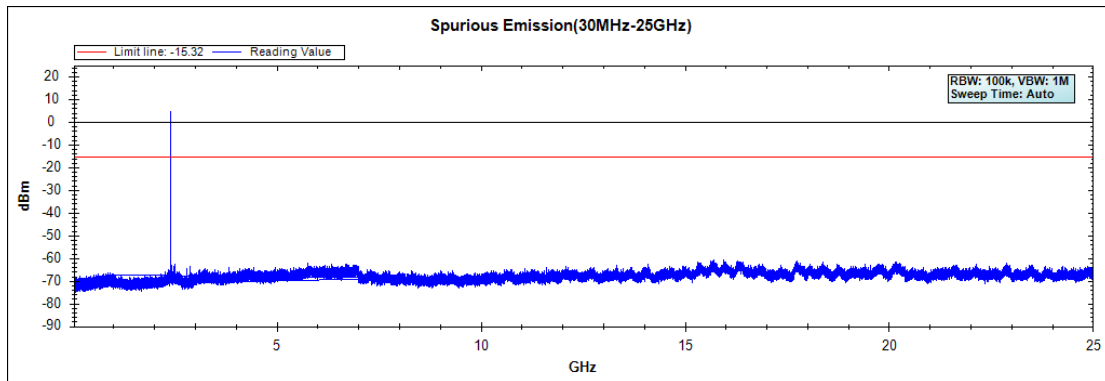
Channel 00 (30MHz-25GHz)-GFSK
