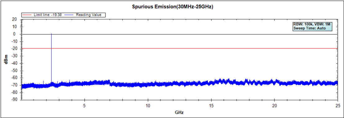
Channel 00 (30MHz-25GHz)-8-DPSK
