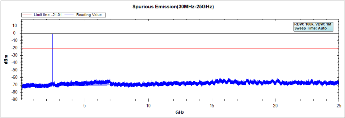
Channel 78 (30MHz-25GHz)-8-DPSK
