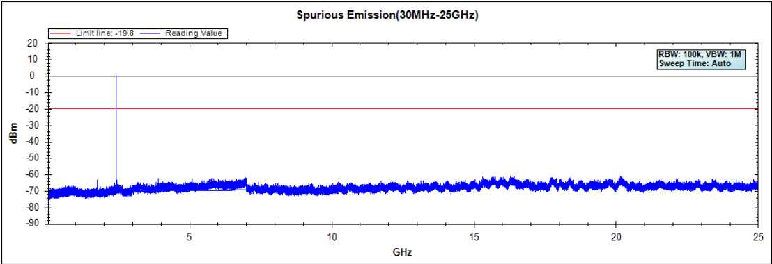
Channel 39 (30MHz-25GHz)-8-DPSK
