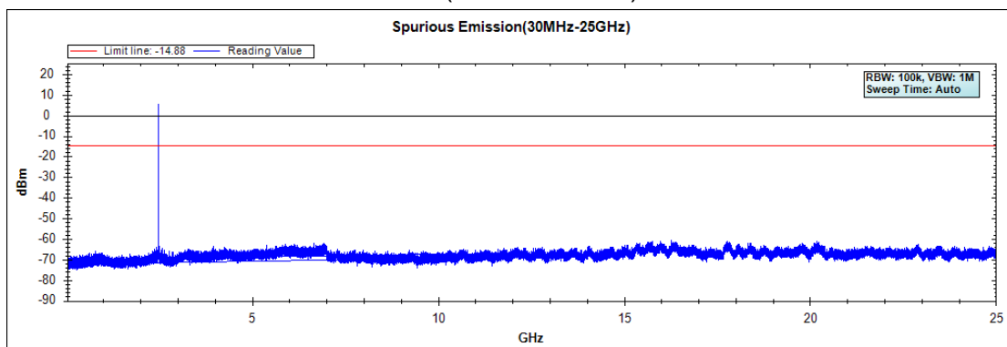
Channel 78 (30MHz-25GHz)-GFSK
