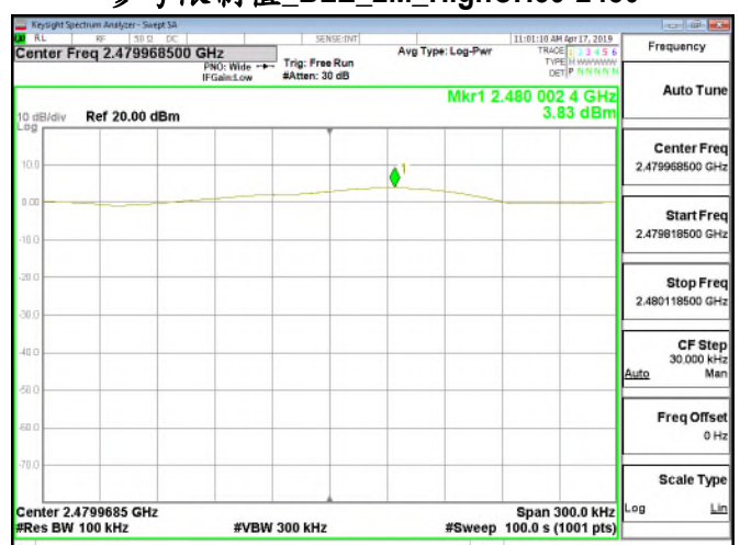
參考限制值_BLE_2M_HighCH39-2480
