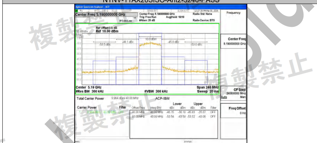
NTNV-11AX40SISO-Ant1-5190-PASS
