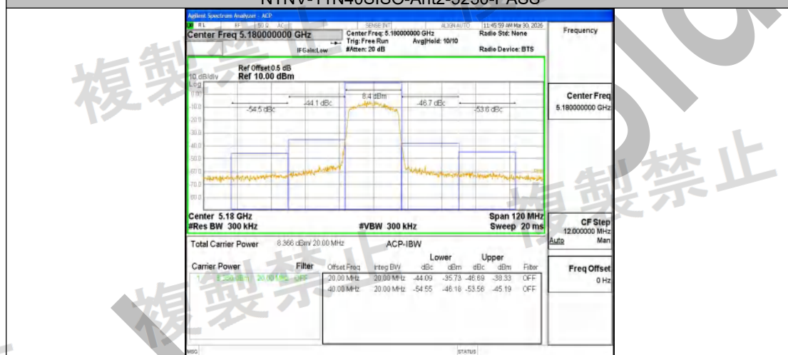
NTNV-11AC20SISO-Ant1-5180-PASS
