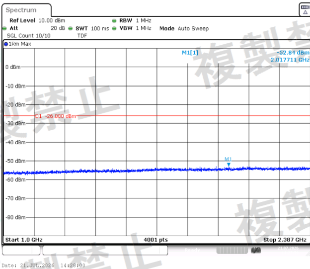
NTVN-BLE_2M-Ant1-2402-1000~2387-PASS
