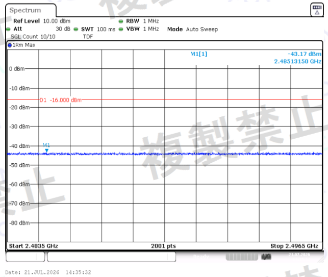
NTNV-BLE_2M-Ant1-2440-2483.5~2496.5-PASS
