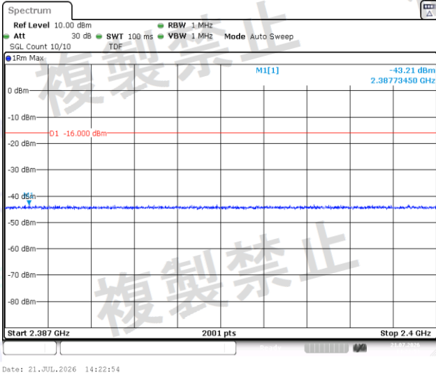
NTVN-BLE_1M-Ant1-2480-2387~2400-PASS
