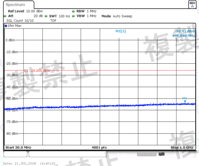
NTNV-BLE_2M-Ant1-2480-30~1000-PASS
