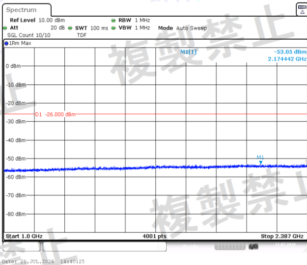
NTNV-BLE_2M-Ant1-2480-1000~2387-PASS
