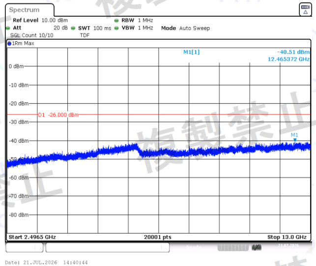
NTNV-BLE_2M-Ant1-2480-2496.5~13000-PASS
