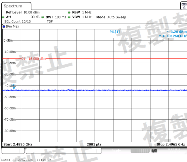
NTNV-BLE_2M-Ant1-2480-2483.5~2496.5-PASS
