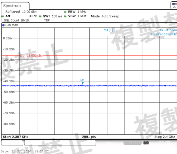
NTNV-BLE_2M-Ant1-2440-2387~2400-PASS
