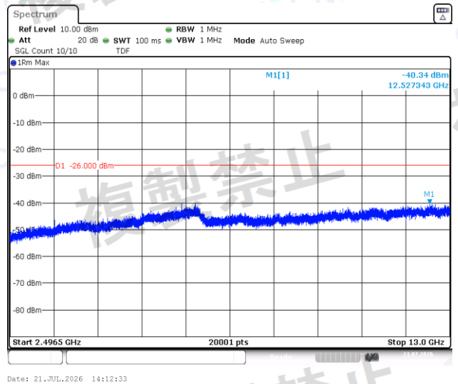
NTNV-BLE_1M-Ant1-2440-2496.5~13000-PASS
