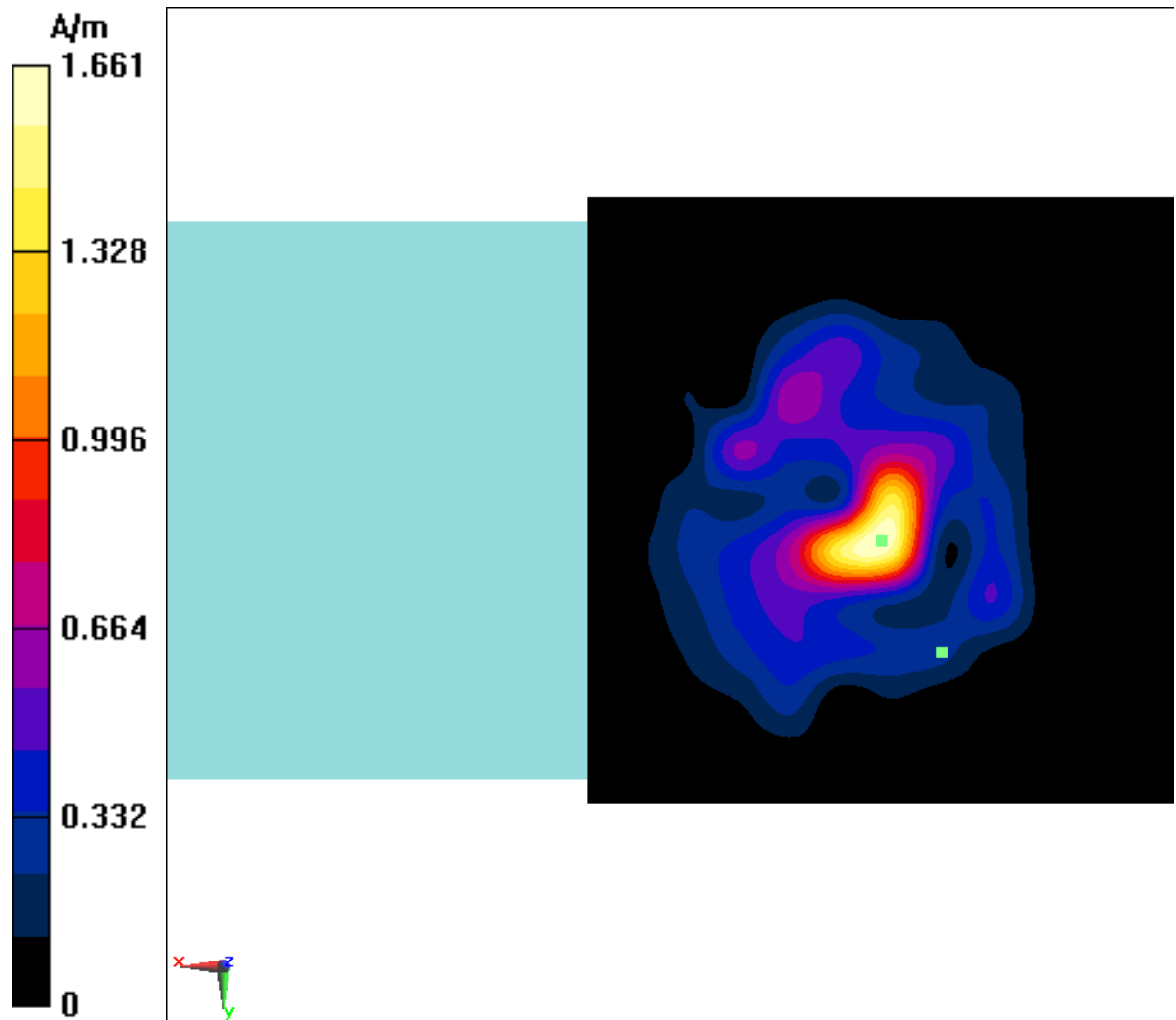
Fig B.4 T-Coil GSM 1900
