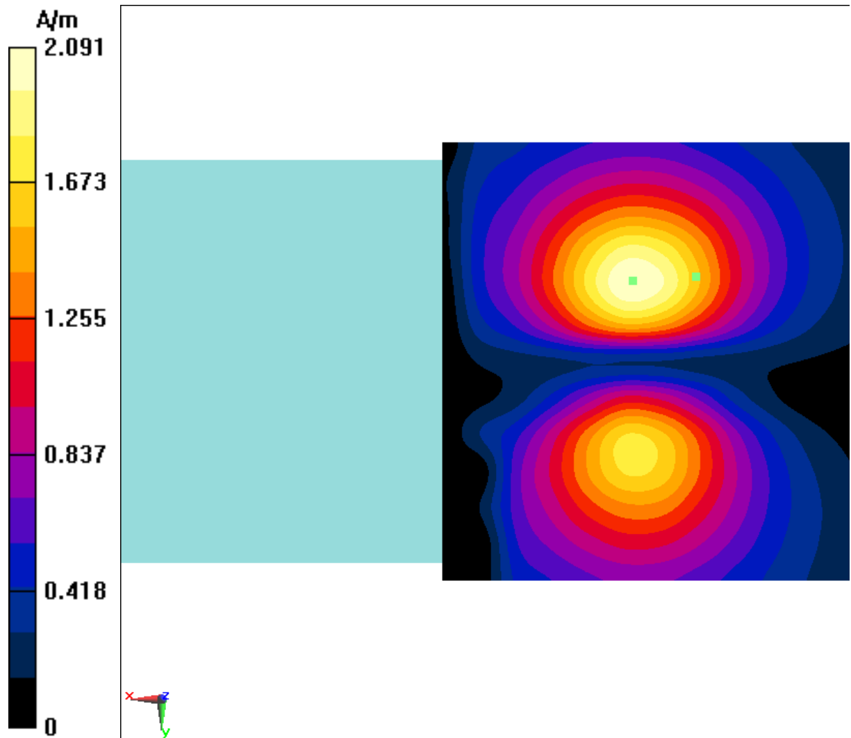
Fig B.3 T-Coil GSM 1900
