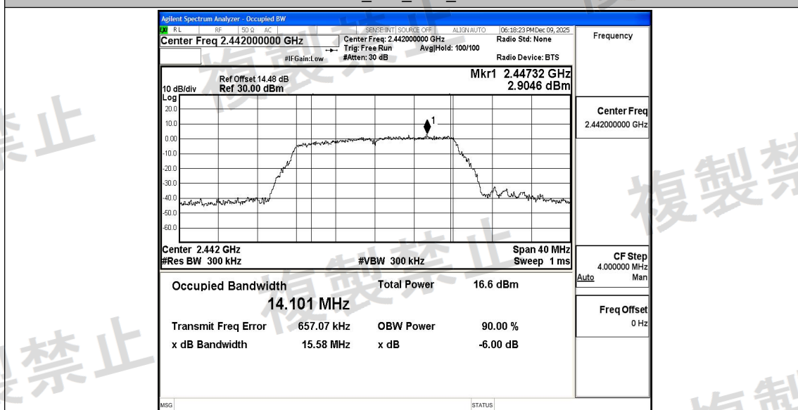
NTNV_11G_Ant1_2442
