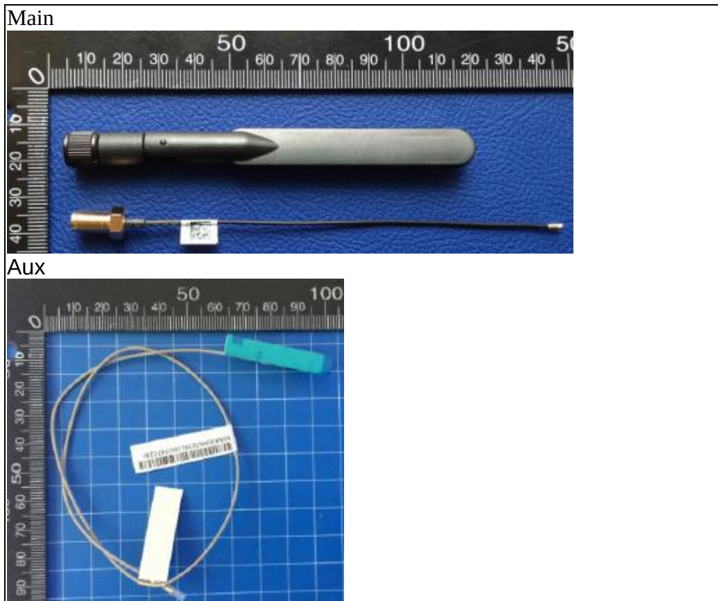
Antenna 8. L01RF031-DT-R+L01RF062-DT-R(Main), L01RF095-DT-R(Aux), Luxshare-ICT Corporation, 2017/06/21
