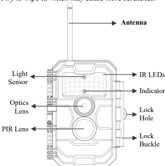
Figure 1: Front View
