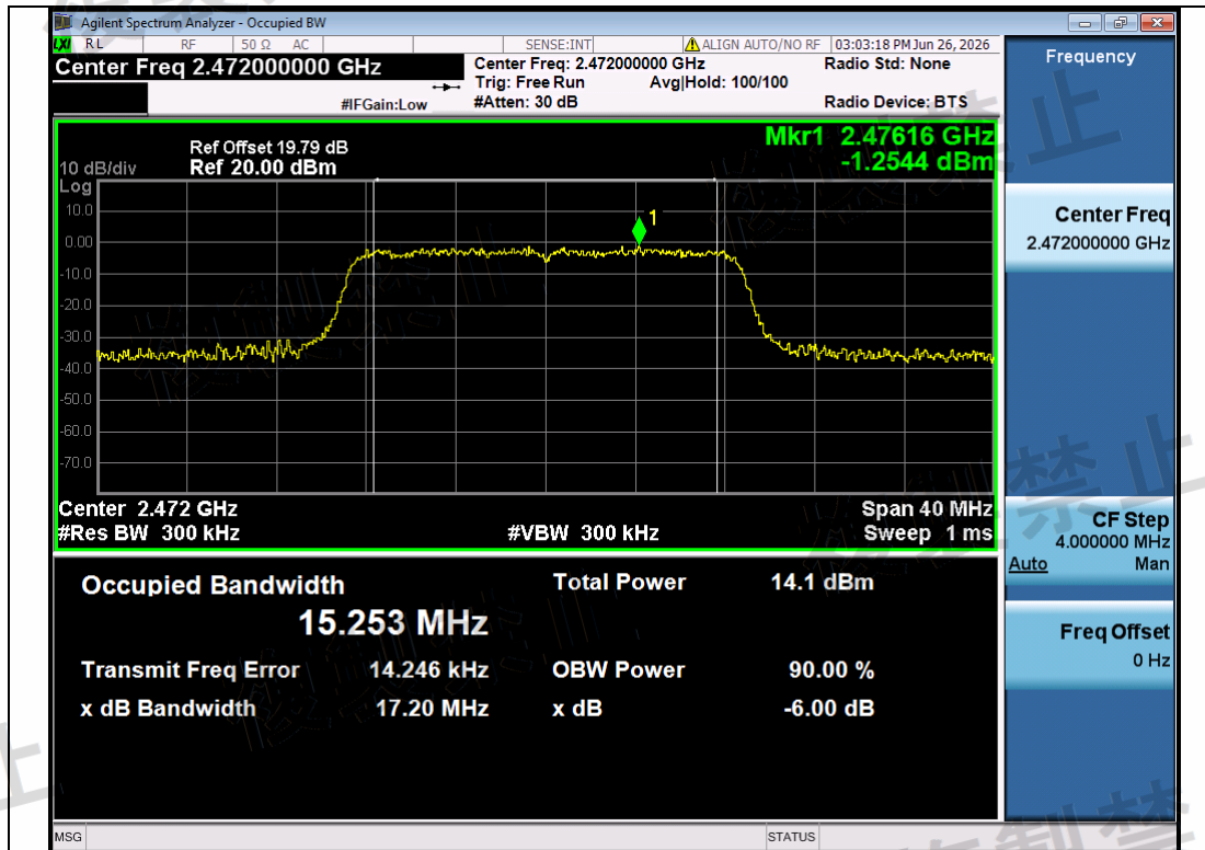
NTNV-11N20SISO-Ant1-2472-PASS
