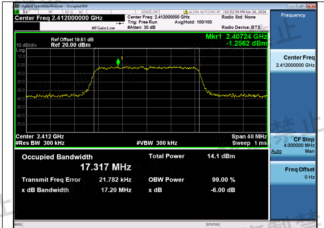
NTNV-11N20SISO-Ant1-2412-PASS
