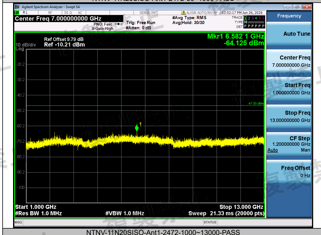
NTNV-11N20SISO-Ant1-2472-1000~13000-PASS
