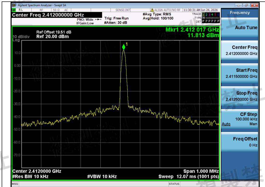
NTNV-11B-Ant1-2412-PASS
