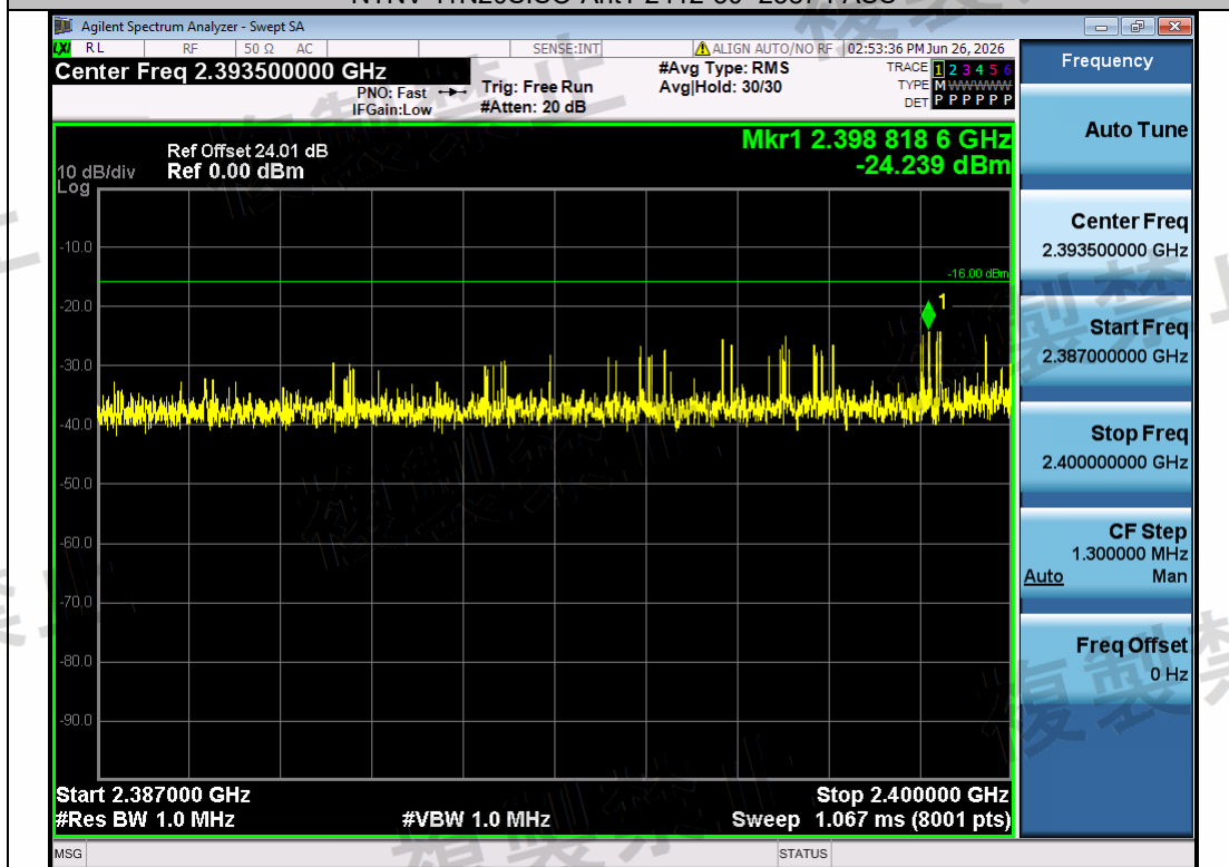
NTNV-11N20SISO-Ant1-2412-2387~2400-PASS
