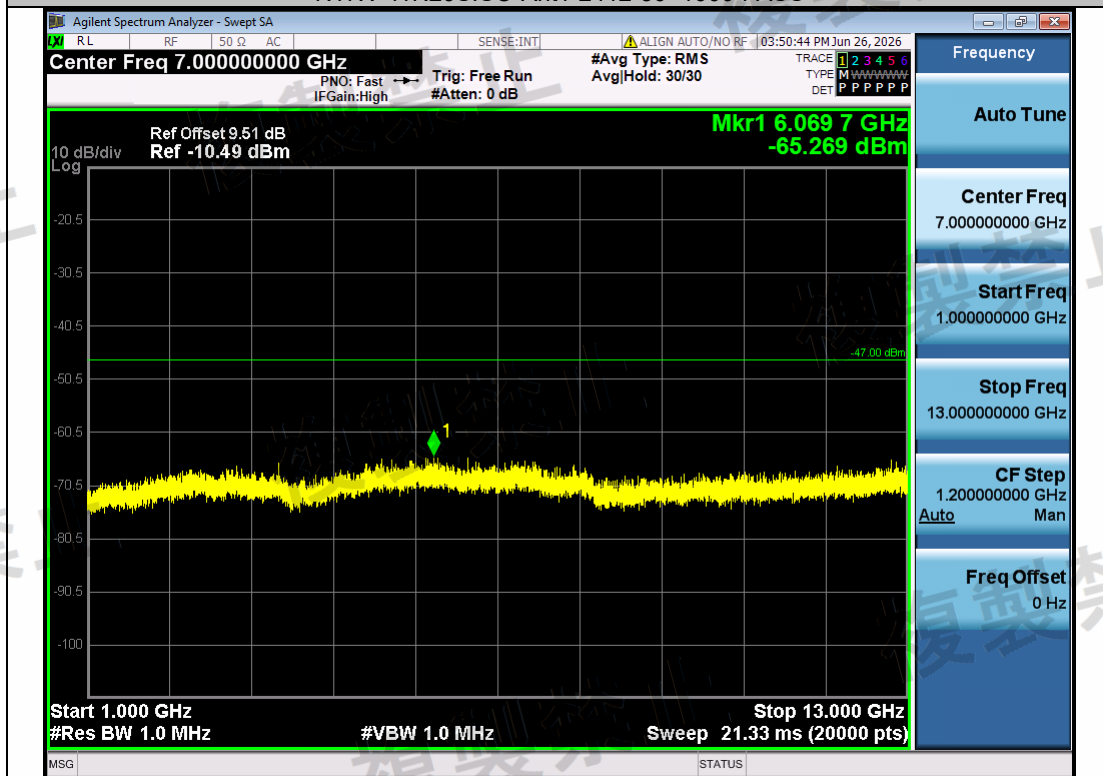
NTNV-11N20SISO-Ant1-2412-1000~13000-PASS
