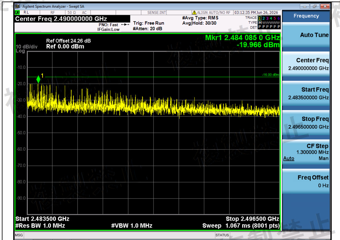
NTNV-11N20SISO-Ant1-2472-2483.5~2496.5-PASS
