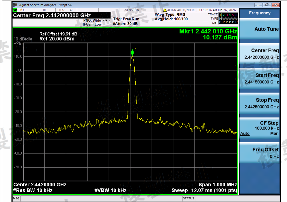
NTNV-11B-Ant1-2442-PASS
