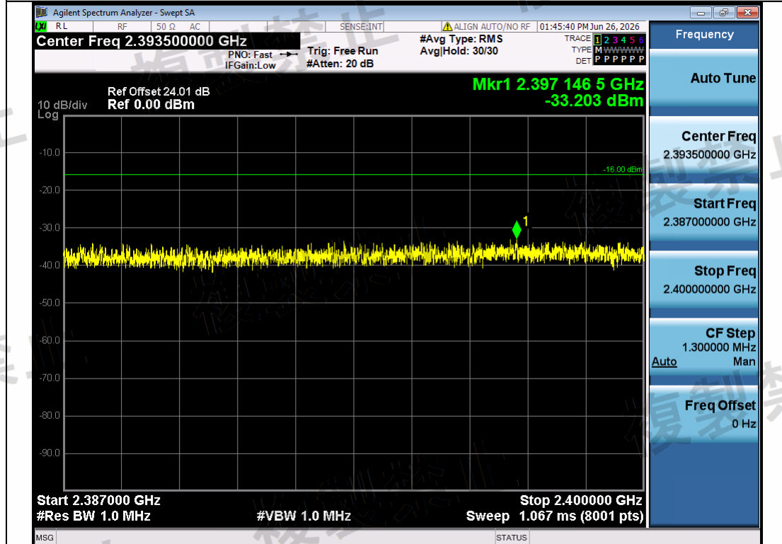
NTNV-11B-Ant1-2412-2387~2400-PASS
