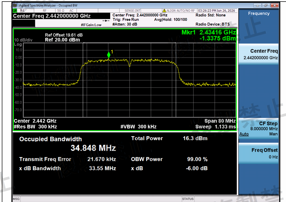
NTNV-11N40SISO-Ant1-2442-PASS
