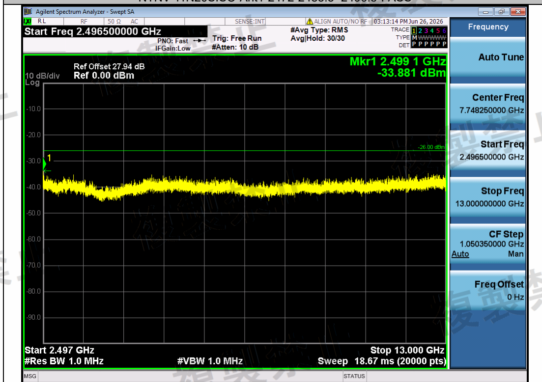
NTNV-11N20SISO-Ant1-2472-2496.5~13000-PASS
