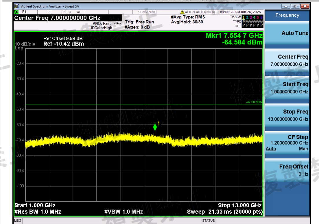
NTNV-11N40SISO-Ant1-2422-1000~13000-PASS
