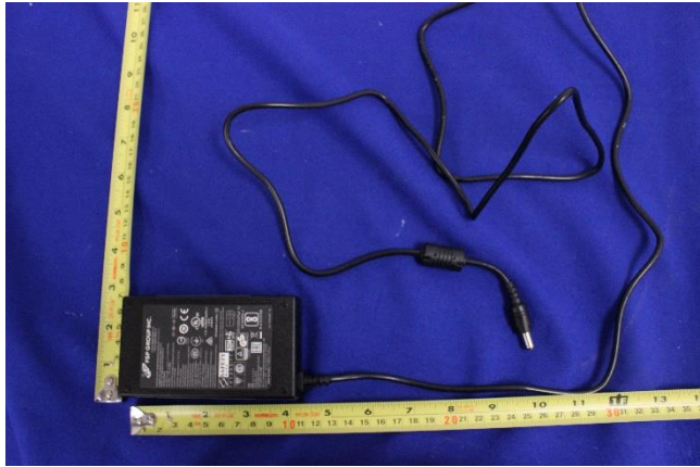
Powersupply View 2
