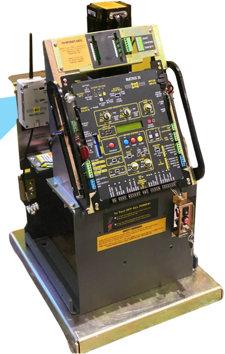
Slide Gate Operator
