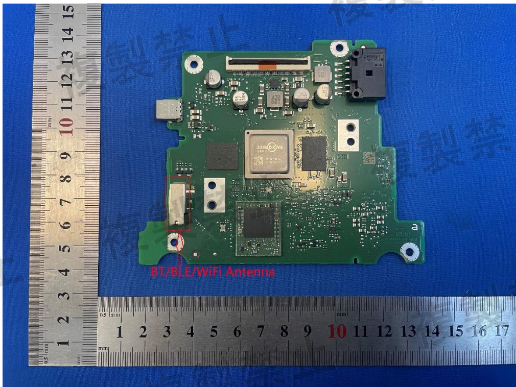
Photo 12: Internal View for BT/BLE/WiFi Antenna
