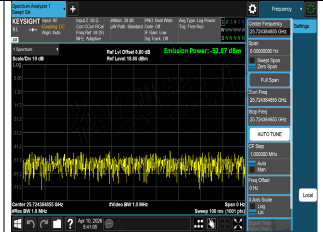
W52 802.11ax 20MHz Chain2 5240MHz Sample 7
