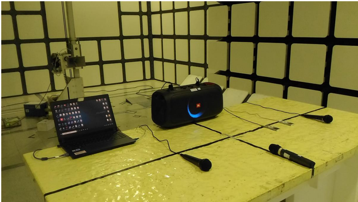
Above 1 GHz _ Rear View
