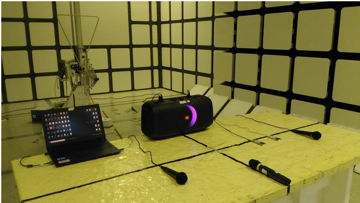
Below 1 GHz _ Rear View
