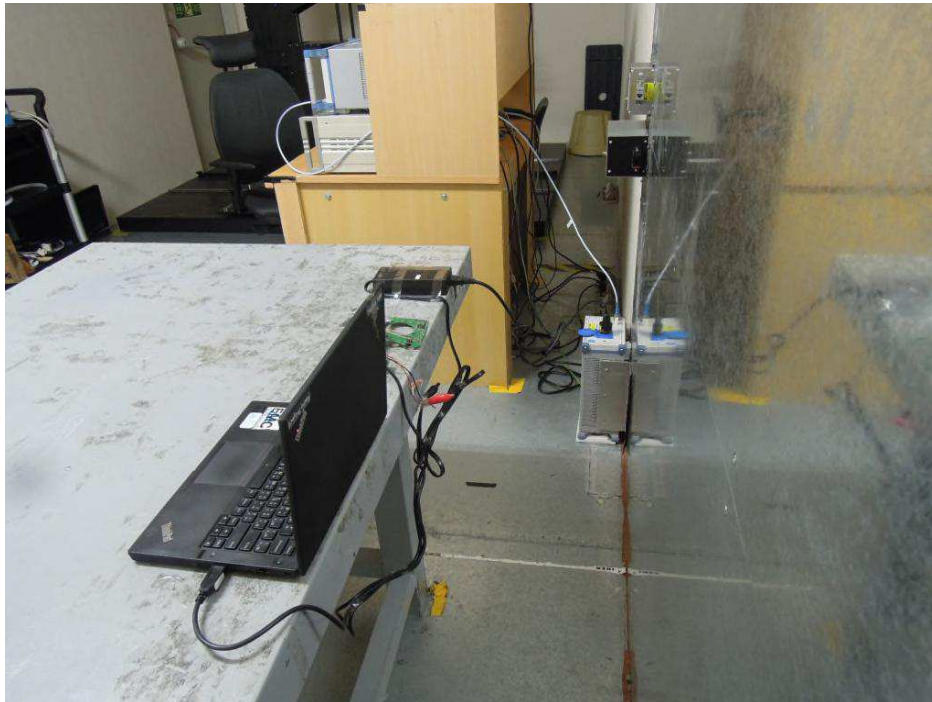
Photograph 12: Set-up for Mains Conducted testing Back, Z10NE030
