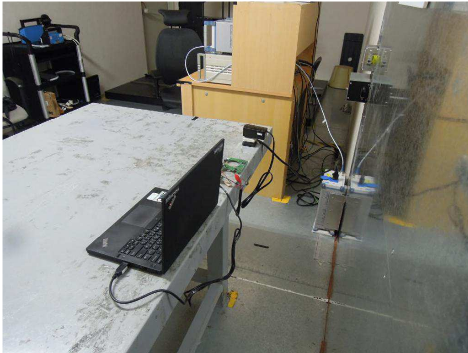
Photograph 10: Set-up for Mains Conducted testing Back, Z10NA300
