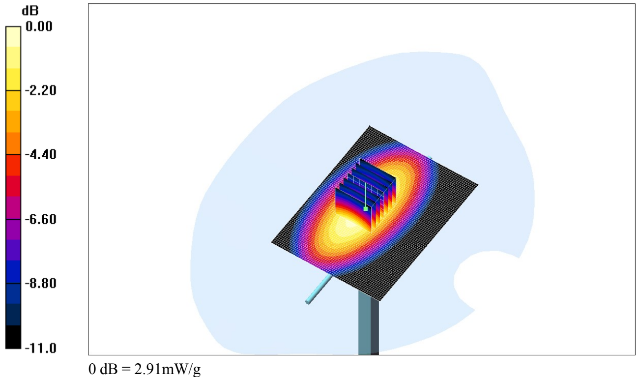
Fig. 8: 900 MHz validation result Meas. Date: Nov. 13, 2012
