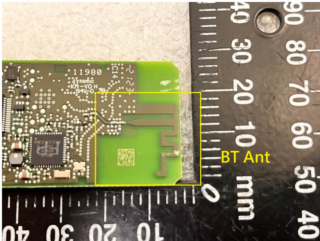
EUT-18. BT Ant
