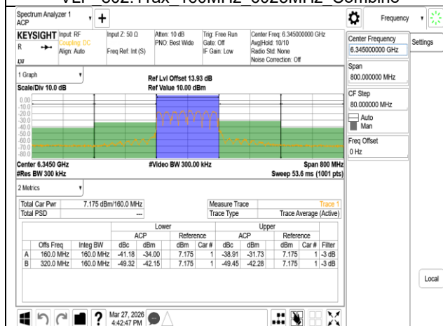
VLP 802.11ax 160MHz 6345MHz Combine
