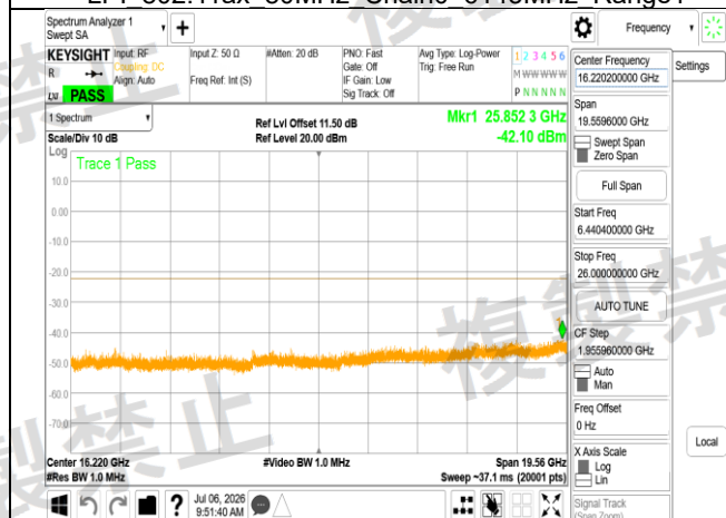
LPI 802.11ax 80MHz Chain0 6145MHz Range3
