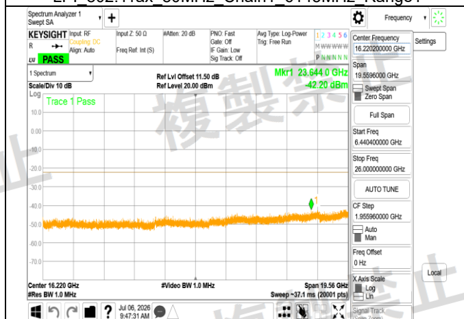
LPI 802.11ax 80MHz Chain1 6145MHz Range3
