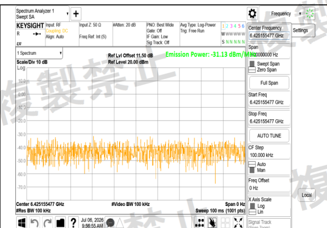
LPI 802.11ax 80MHz Chain0 6385MHz Range2_Sample
