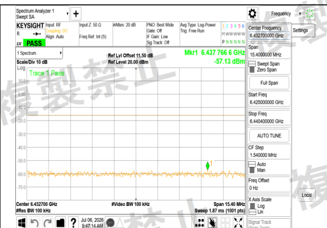
LPI 802.11ax 80MHz Chain1 6145MHz Range2
