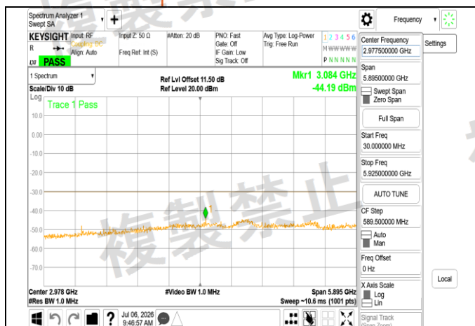
LPI 802.11ax 80MHz Chain1 6145MHz Range1
