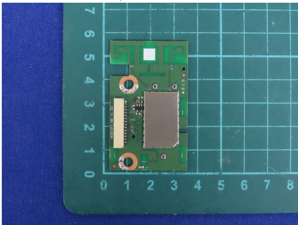
(1) EUT Photo - Trade Name: Hisense, Model No.: MW510-1
