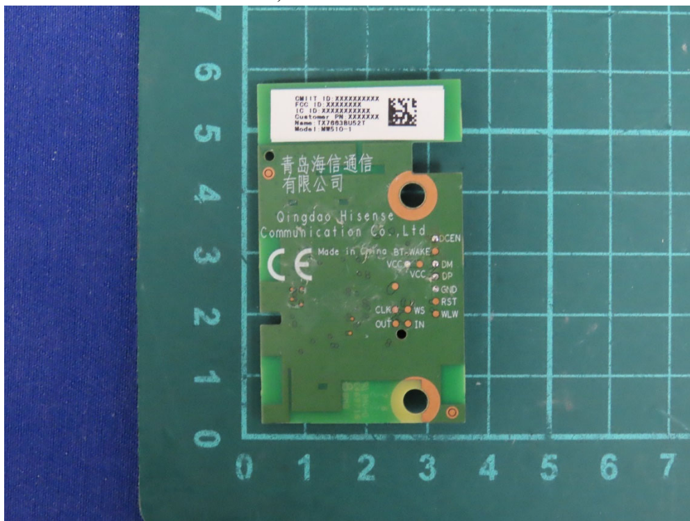
(2) EUT Photo - Trade Name: Hisense, Model No.: MW510-1
