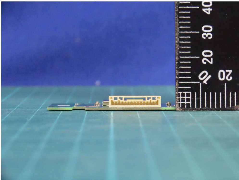
(6) EUT Photo - Trade Name: Hisense, Model No.: MW510-1
