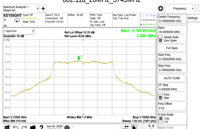
802.11a_20MHz_5745MHz
