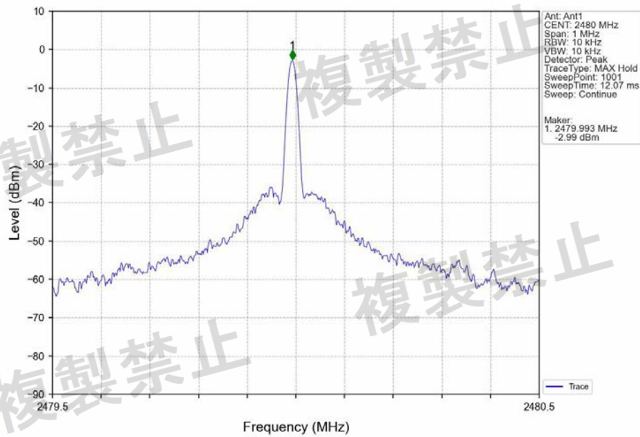
Frequency Error_NTNV_Carrier Wave_2480MHz_Ant1_NTNV
