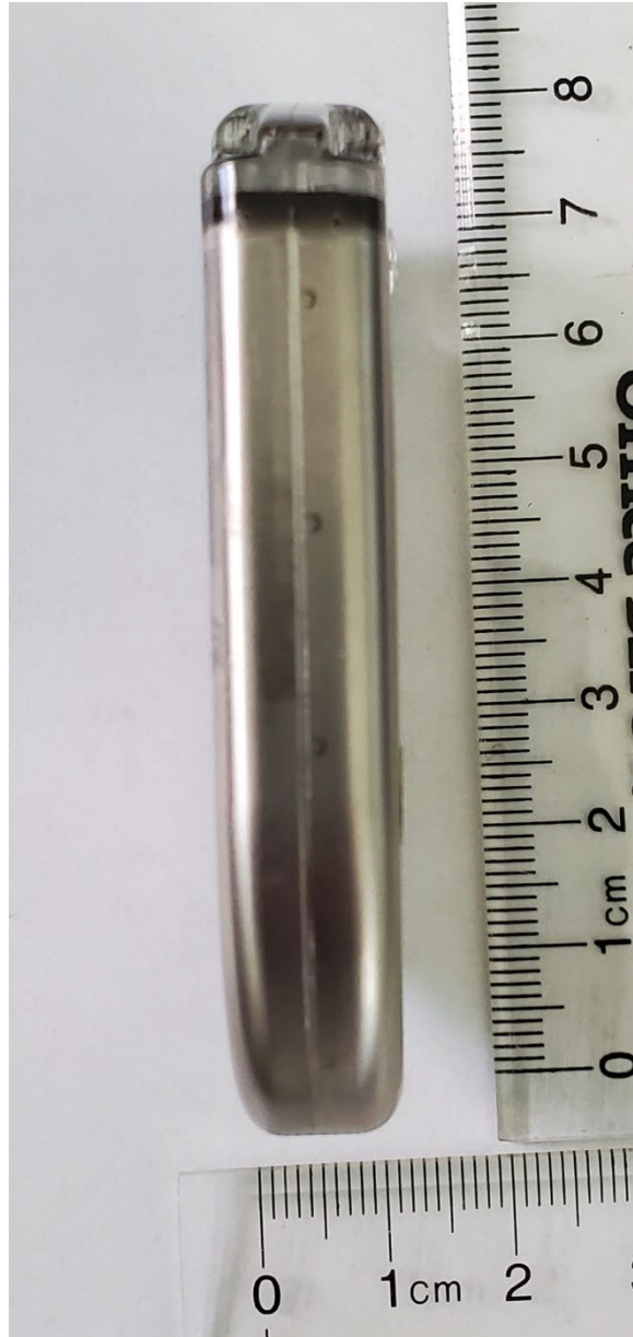
Figure 6: 16 Electrode Blink IPG External Photo – Side
