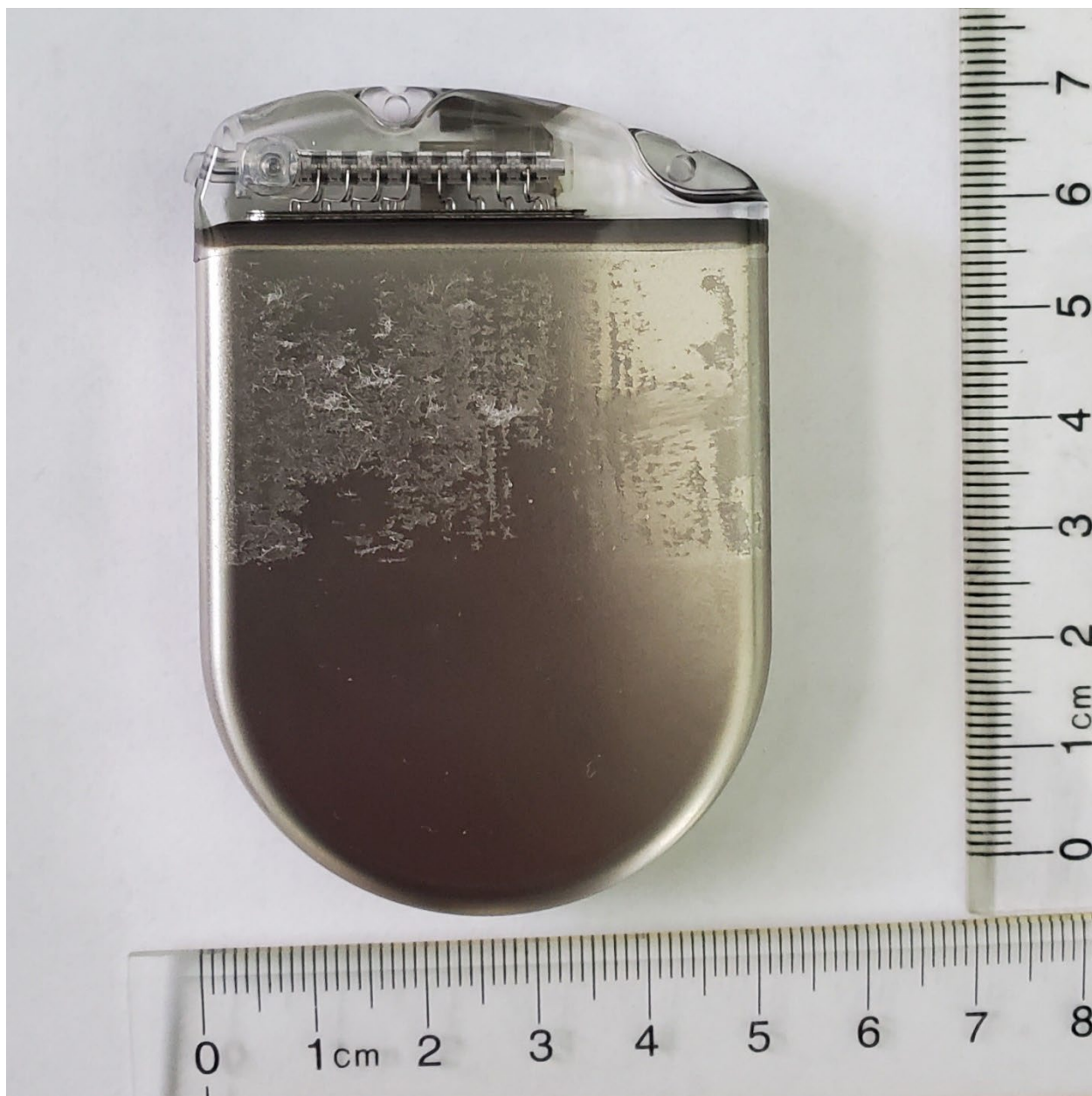
Figure 3: 16 Electrode Blink IPG External Photo – Backside
