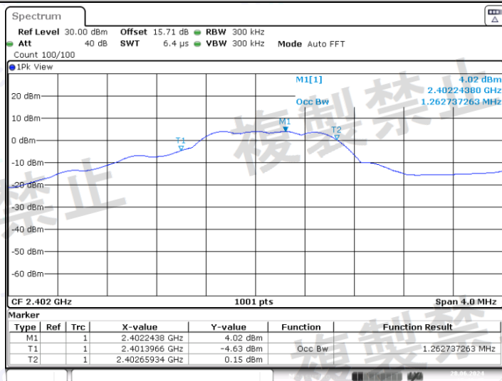
NTNV_BLE_1M_Ant1_2402
