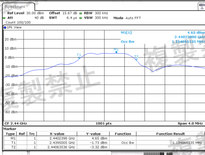
NTNV_BLE_1M_Ant1_2440
