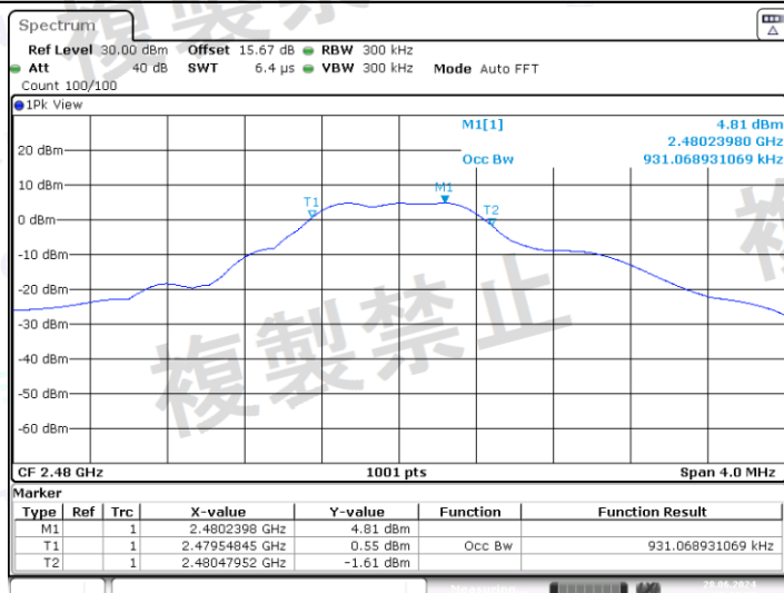
NTNV_BLE_1M_Ant1_2480
