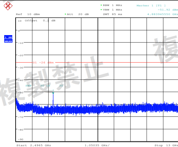
NTNV_11B_Ant1_2442_2496.5~13000
