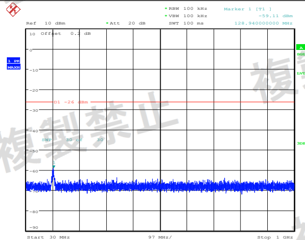
NTNV_11N20SISO_Ant1_2442_30~1000
