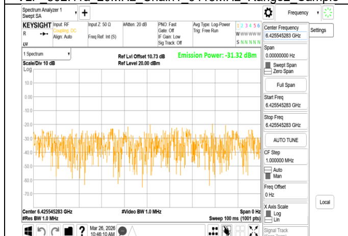
VLP_802.11a_20MHz_Chain1_6415MHz_Range3_Sample
