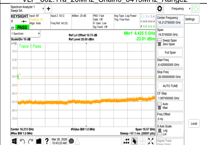
VLP_802.11a_20MHz_Chain0_6415MHz_Range3
