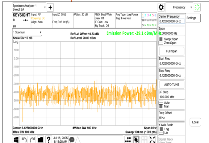
LPI 802.11be 80MHz Chain1 6385MHz Range2 Sample
