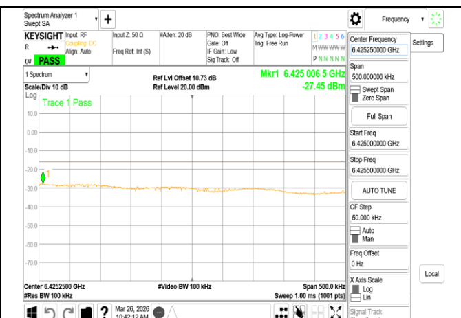
VLP_802.11a_20MHz_Chain1_6415MHz_Range2
