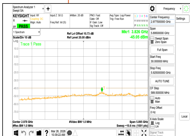
VLP_802.11a_20MHz_Chain0_6415MHz_Range1
