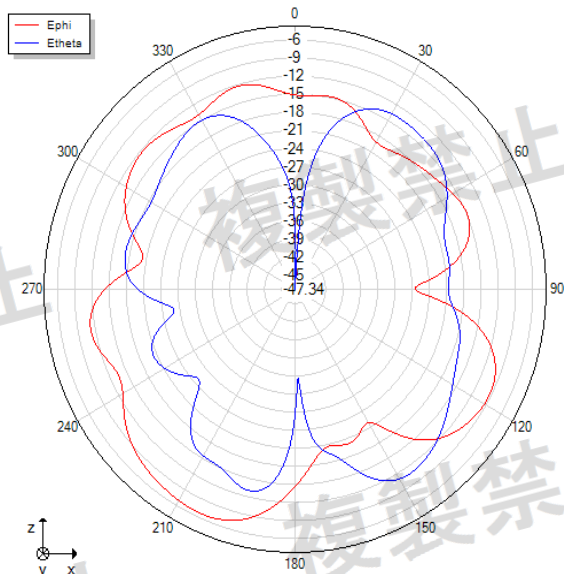
Phi=0 freq=2470MHz
