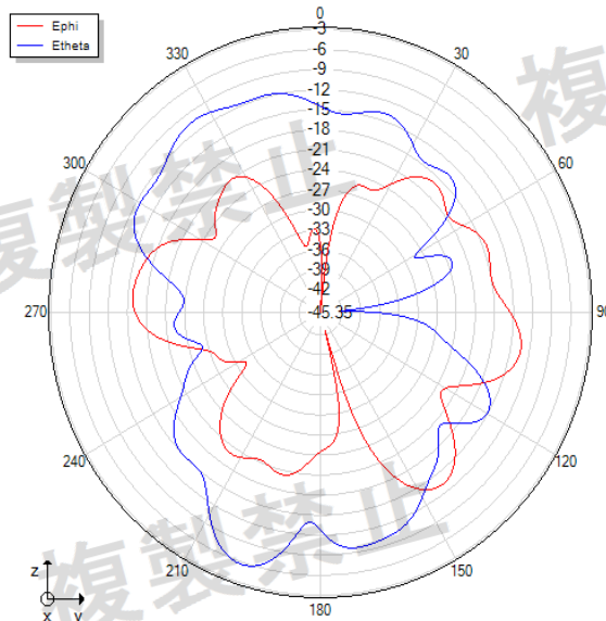
Phi=90 freq=2460MHz
