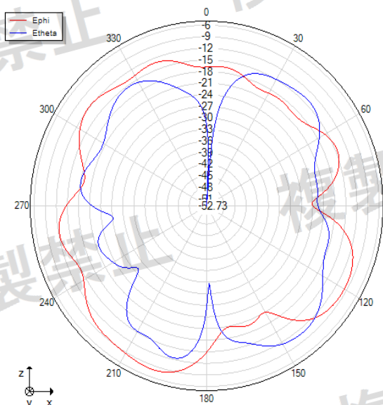
Phi=0 freq=2500MHz
