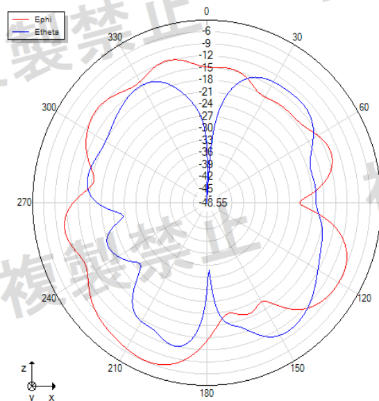
Phi=0 freq=2480MHz
