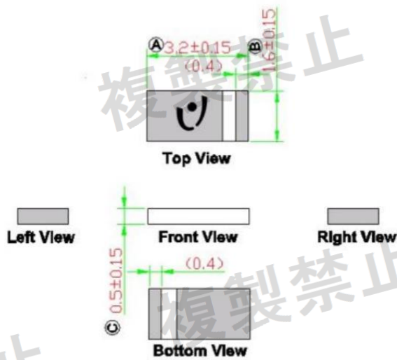
6-1. Antenna Dimensions
