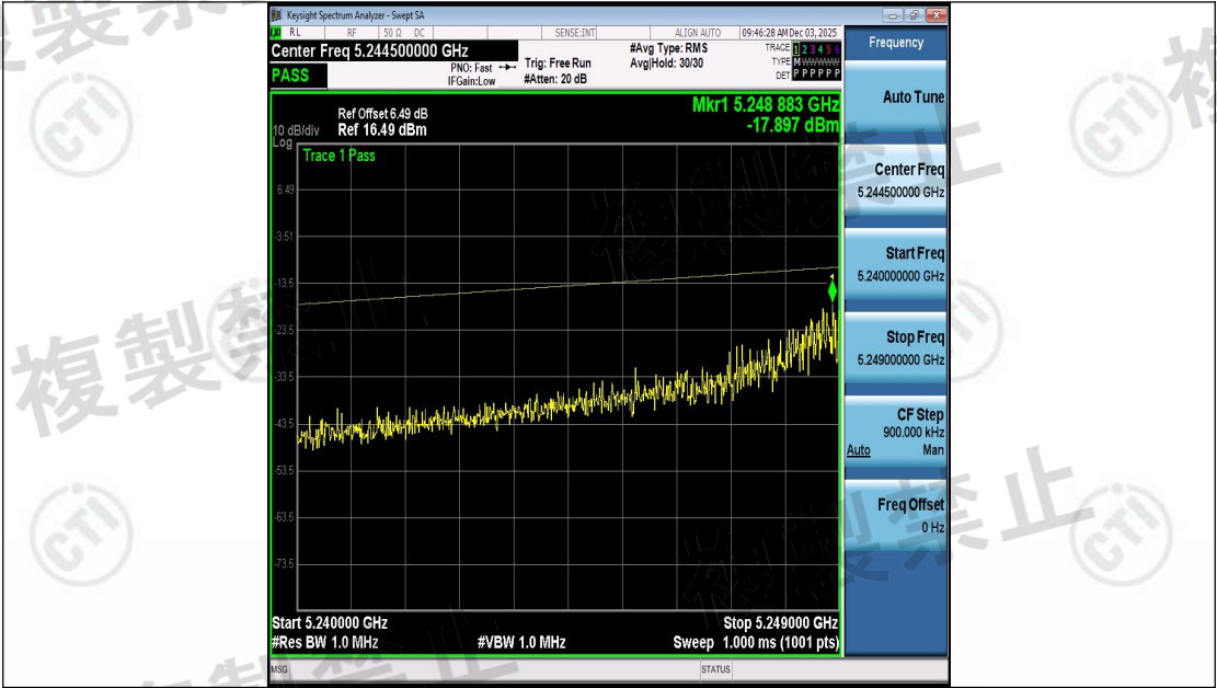
NTNV-11AX20SISO-Ant2-5260-5240~5249-See table below
