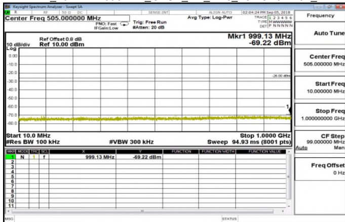
TX 10MHz~1000MHz_GFSK 1M_DH5 LowCH0-2402 1
