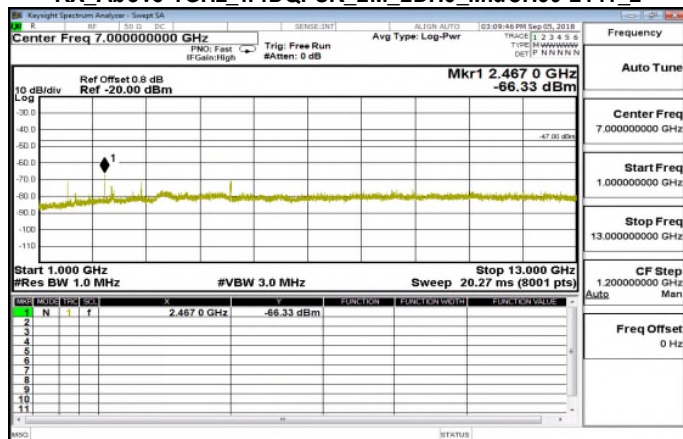
RX_Above 1GHz_π4DQPSK_2M_2DH5_MidCH39-2441_2
