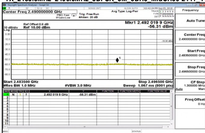
TX 2483.5MHz~2496.5MHz_8DPSK_3M_3DH5_MidCH39-2441_4
