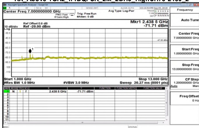
RX_Above 1GHz_π4DQPSK_2M_2DH5_HighCH78-2480_2
