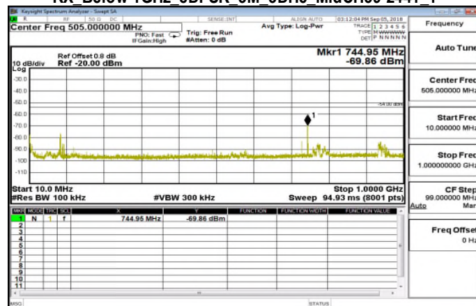
RX_Below 1GHz_8DPSK_3M_3DH5_MidCH39-2441_1
