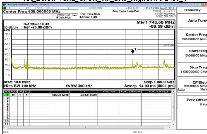
RX Below 1GHz_GFSK_1M_DH5_HighCH78-2480_1
