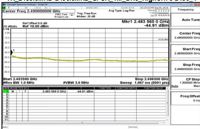
TX 2483.5MHz~2496.5MHz GFSK 1M DH5 HighCH78-2480 4
