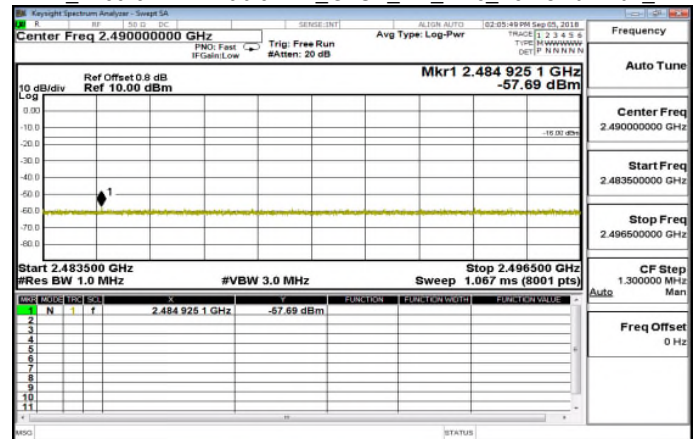
TX 2483.5MHz~2496.5MHz_GFSK 1M_DH5 LowCH0-2402 4
