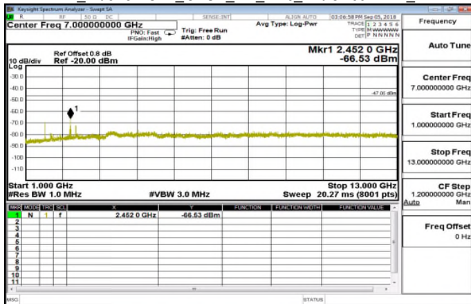
RX Above 1GHz_GFSK_1M_DH5_MidCH39-2441_2
