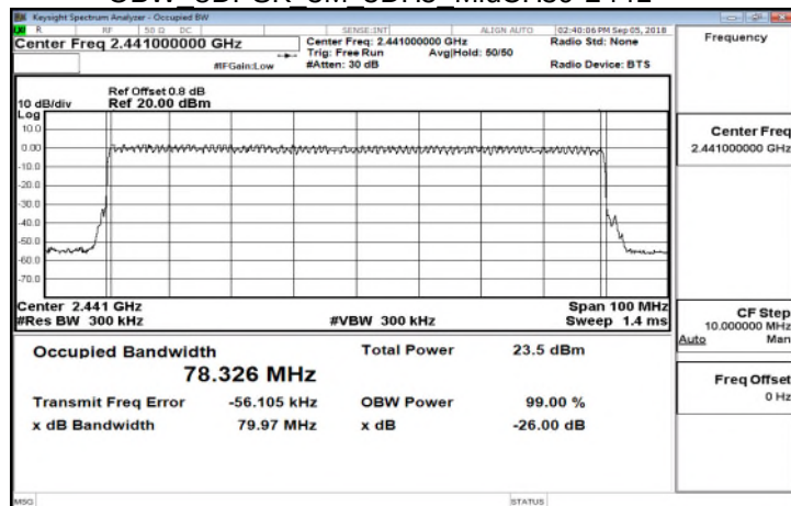
OBW 8DPSK 3M 3DH5 MidCH39-2441
