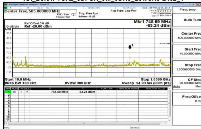
RX_Below 1GHz_8DPSK_3M_3DH5_LowCH0-2402_1
