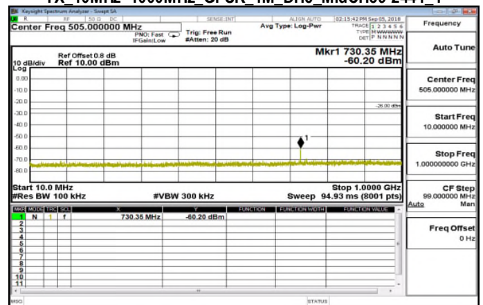
TX 10MHz~1000MHz_GFSK 1M_DH5 MidCH39-2441 1
