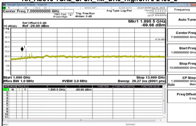
RX Above 1GHz_GFSK_1M_DH5_HighCH78-2480_2
