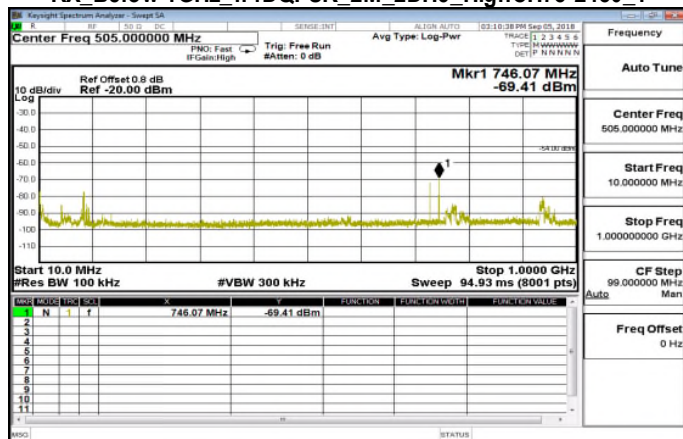
RX_Below 1GHz_π4DQPSK_2M_2DH5_HighCH78-2480_1
