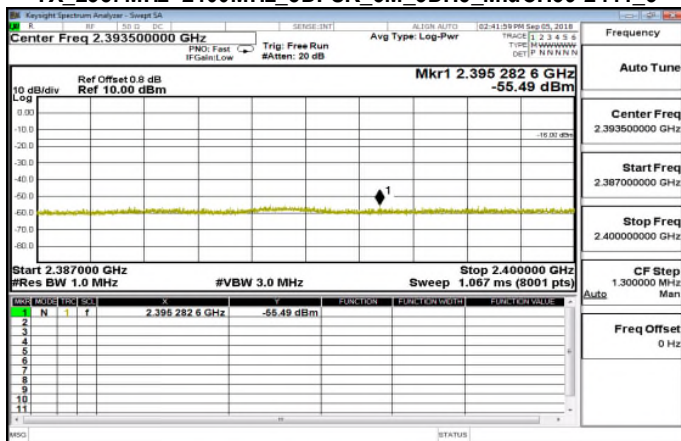
TX 2387MHz~2400MHz_8DPSK_3M_3DH5_MidCH39-2441_3
