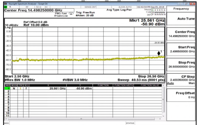
TX 2496.5MHz~26.5GHz_8DPSK_3M_3DH5_MidCH39-2441_5
