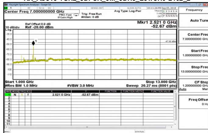
RX_Above 1GHz_8DPSK_3M_3DH5_LowCH0-2402_2
