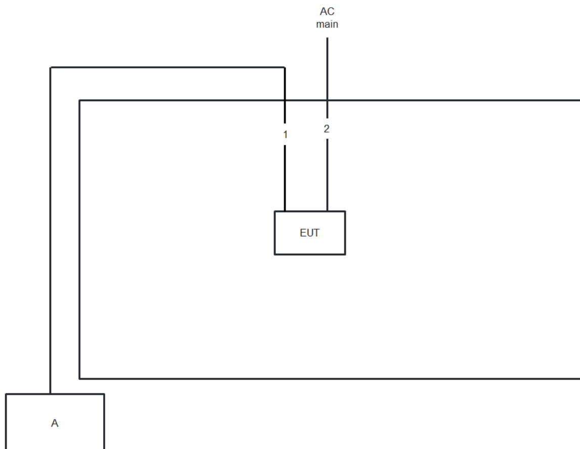
Test Setup Diagram - Radiated Intentional Test
