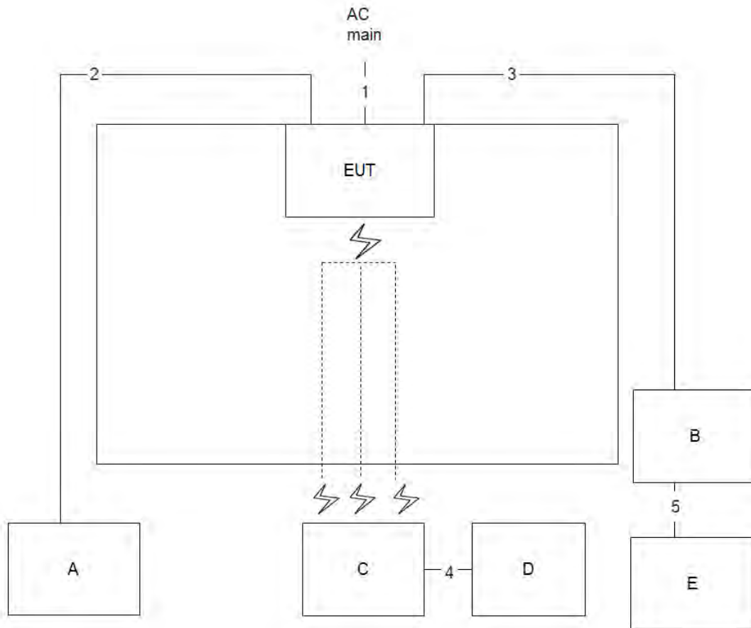
Test Setup Diagram - Radiated Unintentional Test
