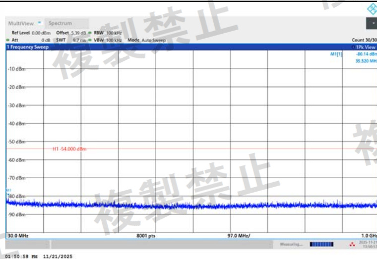
NTNV-DH5-Ant1-2441-30~1000-PASS
