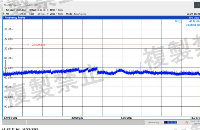
NTNV-2DH5-Ant1-2441-2496.5~13000-PASS
