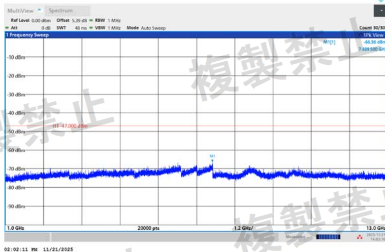
NTNV-3DH5-Ant1-2441-1000~13000-PASS
