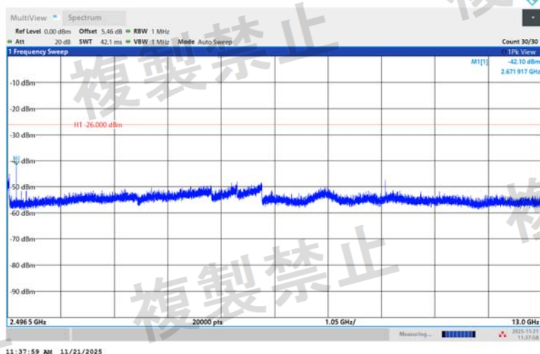
NTVN-3DH5-Ant1-2480-2496.5~13000-PASS
