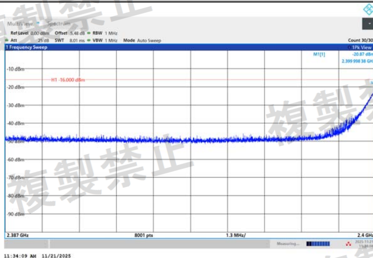
NTVN-3DH5-Ant1-2402-2387~2400-PASS
