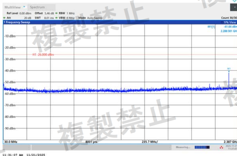
NTNV-2DH5-Ant1-2480-30~2387-PASS
