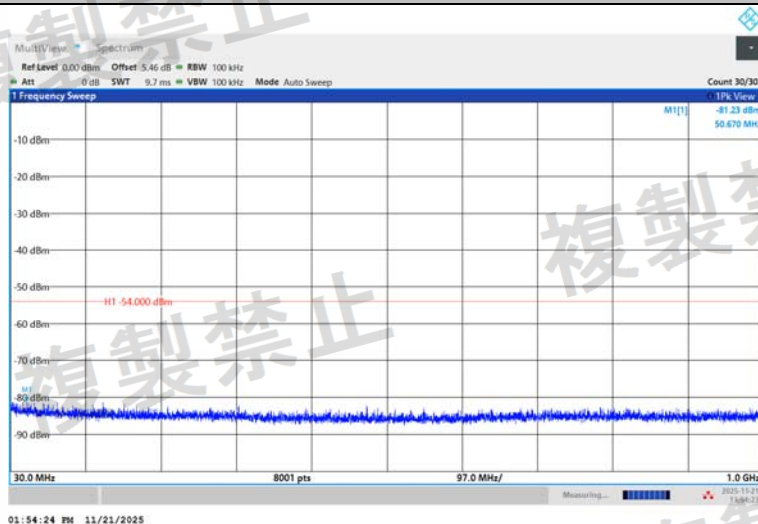
NTV-DH5-Ant1-2480-30~1000-PASS
