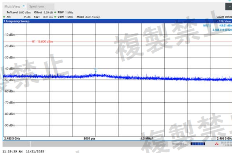
NTNV-2DH5-Ant1-2441-2483.5~2496.5-PASS
