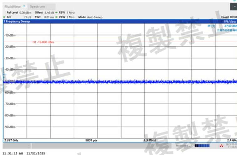
NTVN-2DH5-Ant1-2480-2387~2400-PASS
