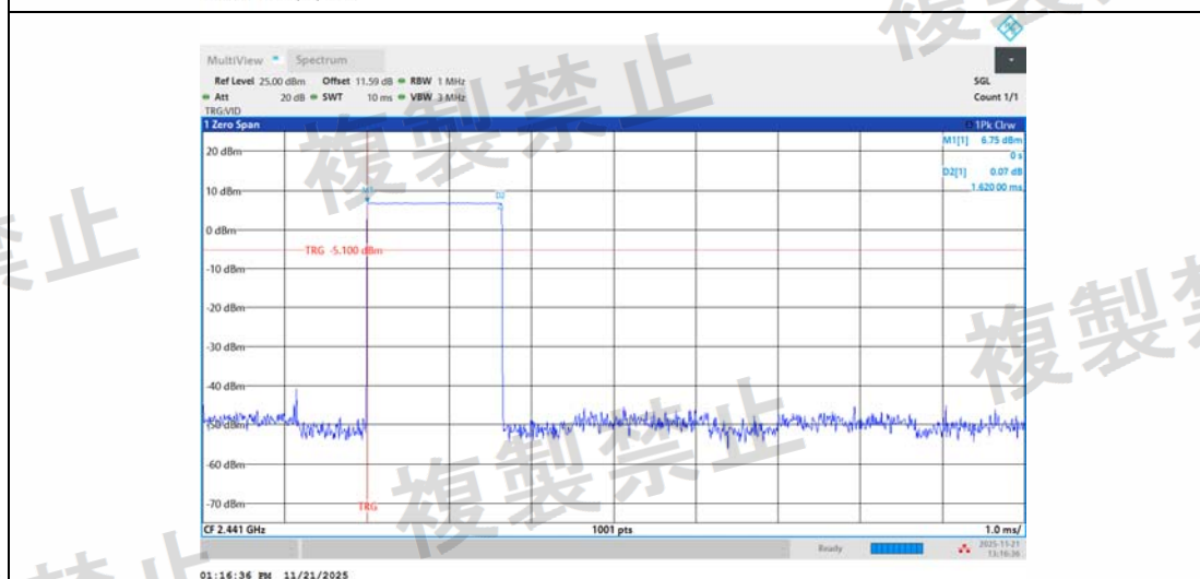
NTNV-DH3-Ant1-Hop-PASS
