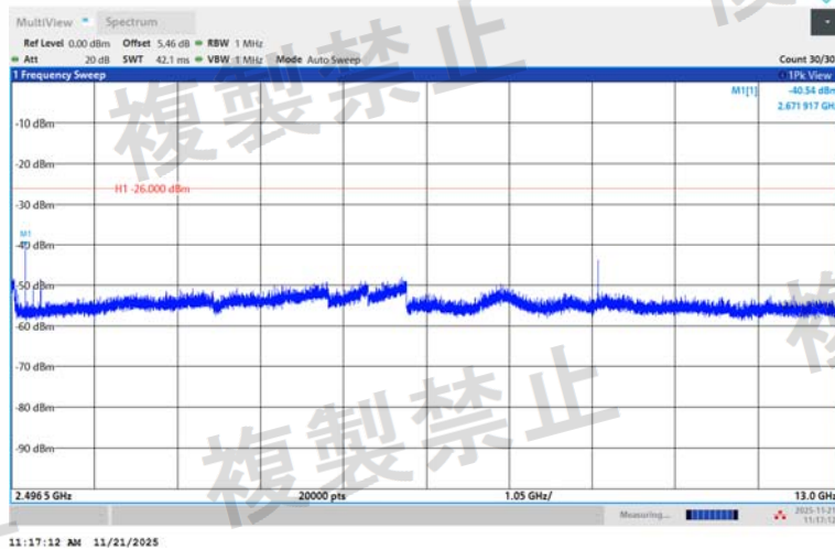
NTNV-DH5-Ant1-2480-2496.5~13000-PASS
