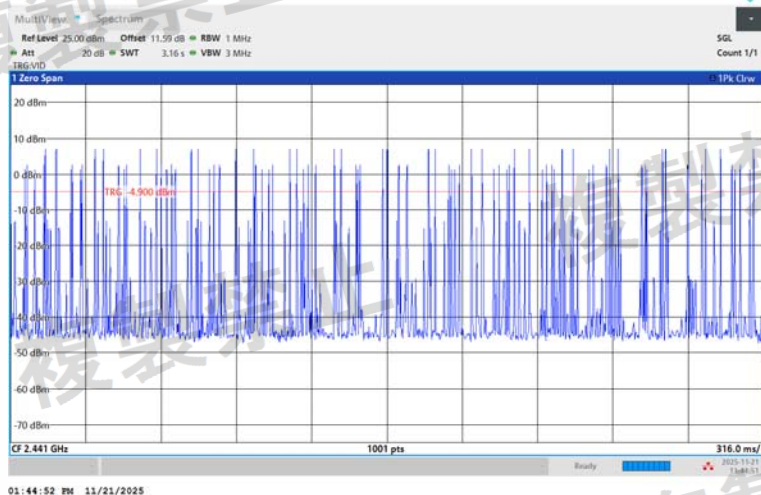
NTNV-3DH1-Ant1-Hop-PASS
