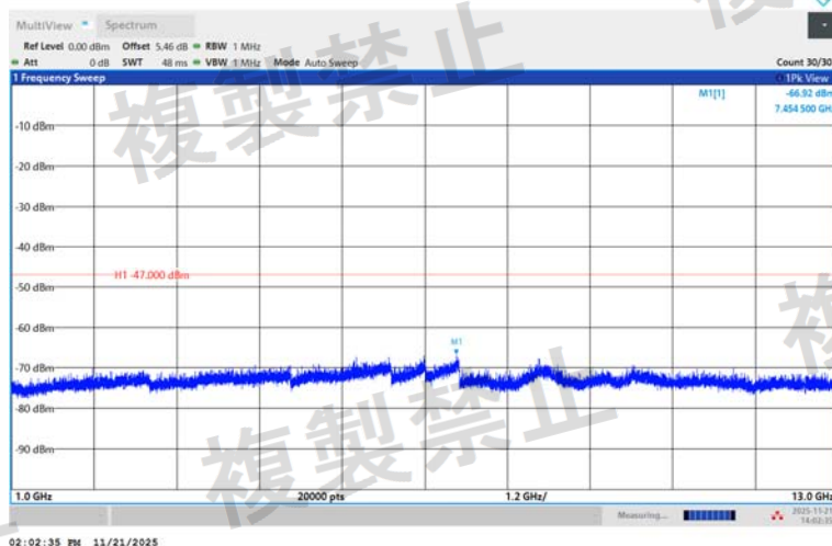
NTNV-3DH5-Ant1-2480-1000~13000-PASS
