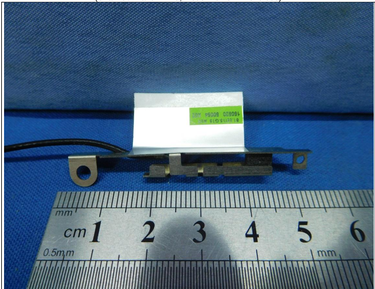
Antenna Set 1 (Chain 0 / Brand: WNC; Model No.: 81-EBJ15.005)
